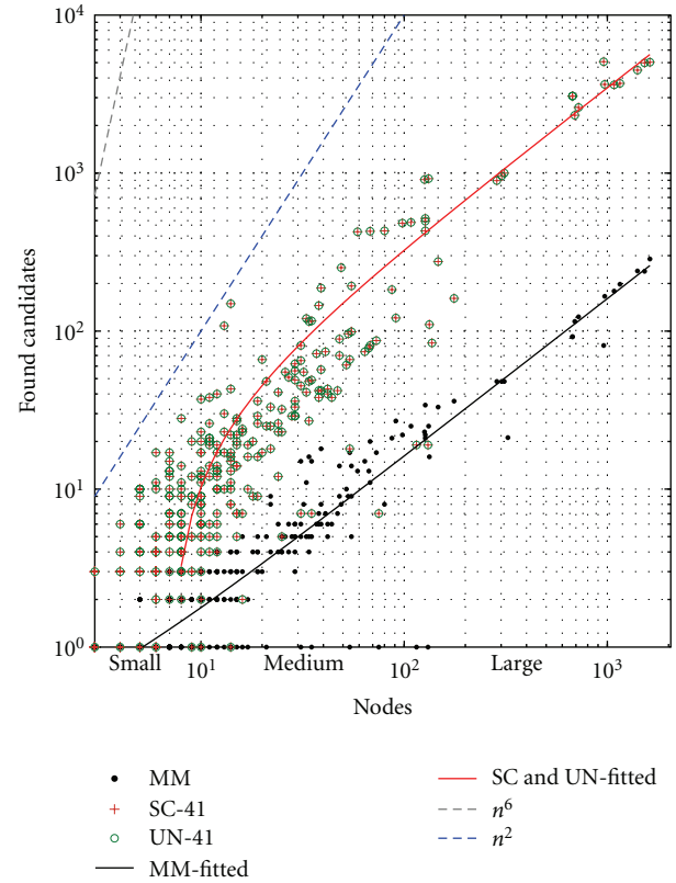
FIGURE 5: Number of found candidates by ISE algorithms for a large spectrum of BB nodes, where SC and UN are constrained to 4 inputs and 1 output.
