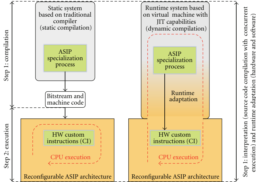
FIGURE 1: Overview of ASIP specialization process for conventional static and runtime systems.
