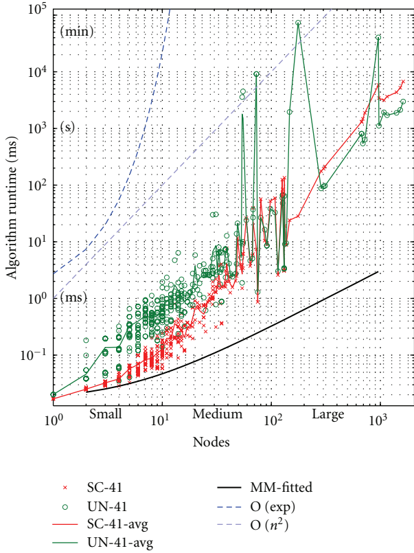
FIGURE 4: Runtimes of the ISE identification algorithm for different basic block sizes (nodes). The SC: SingleCut, UN: Union, MM: MaxMiso algorithms. The label “41” means that the SC and UN search has been constrained to 4 inputs and 1 output.
