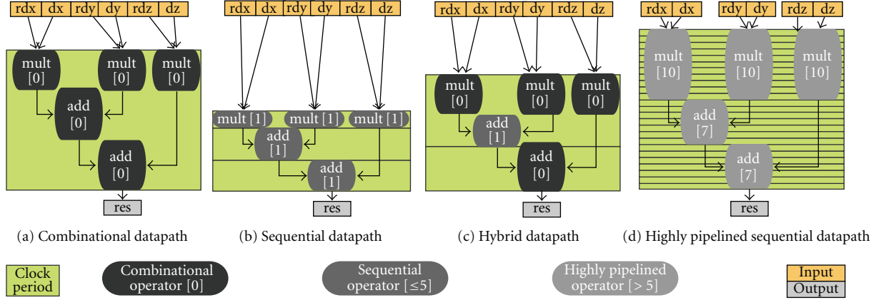
FIGURE 3: Different types of a DFG presented for a UDCI candidate shown in Listing 2.
