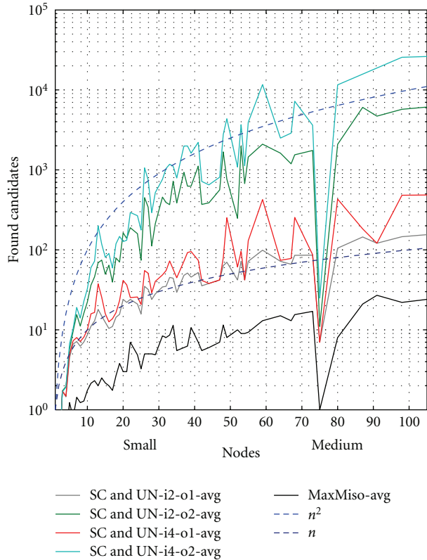
FIGURE 6: Number of found candidates by ISE algorithms for a medium spectrum of BB nodes, where SC and UN have variable constraints.
