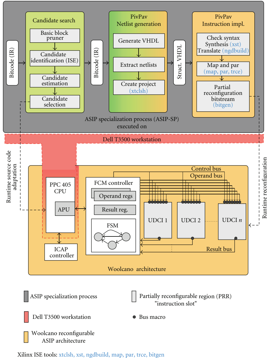
FIGURE 2: Overview of the developed tool flow and the targeted Woolcano hardware architecture. During experimental evaluation, instead of a PPC405 CPU, the ASIP specialization process was executed on a Dell T3500 workstation; see Section 10 for details.
