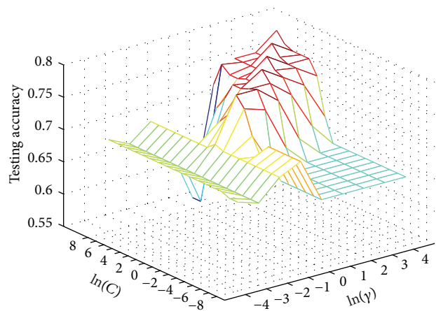
(b) KELM for ionosphere dataset
