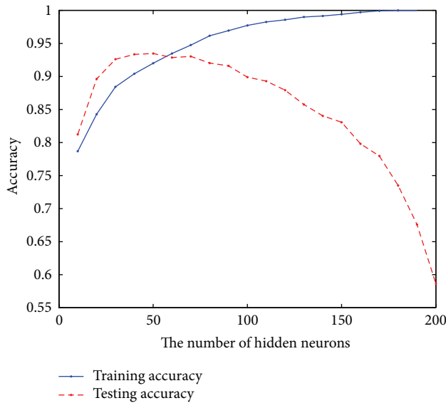
(a) Basic ELM for ionosphere dataset
