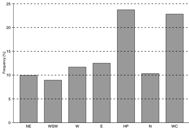
Figure 2. CAP7 1763–2009 JFM mean frequency of occurrence.
