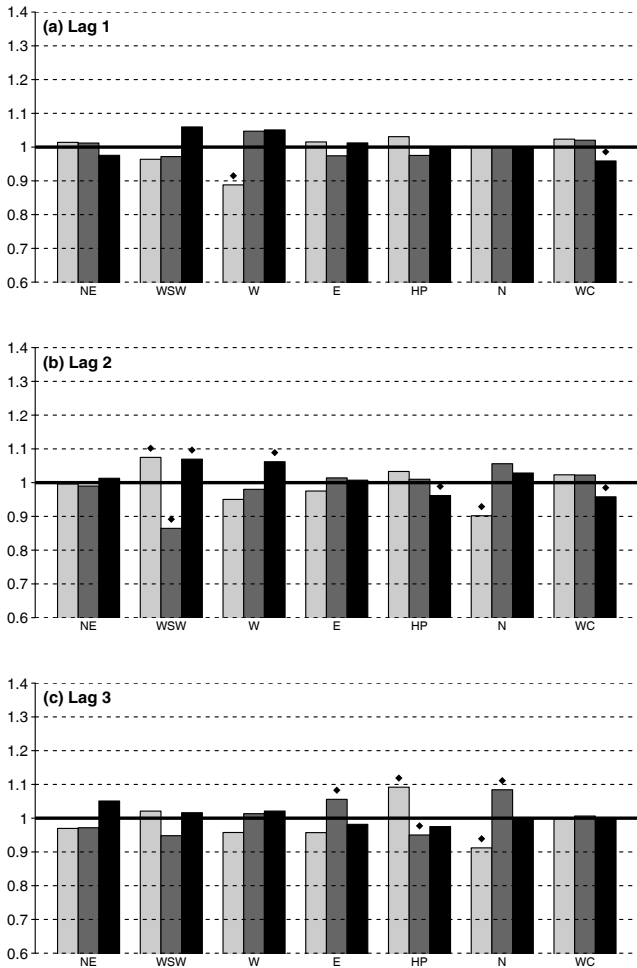
Figure 6. Ratios of the frequency for the low (light grey), moderate (grey), and high (black) solar activity classes for 1-year (a), 2-year (b), and 3-year (c) lags relative to the long-term mean. Dots correspond to statistical significance of the ratios at the 95 % level.
