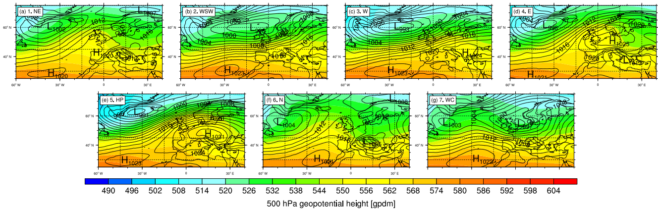
Figure 3. CAP7 1958–2009 500 hPa geopotential height (colour) in gpdm and sea level pressure (contours) in hPa JFM composites.
