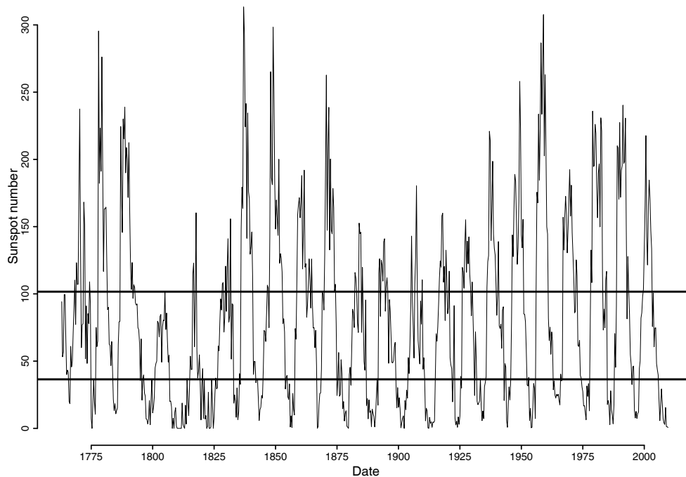
Figure 1. 1763–2009 JFM monthly sunspot number with 33rd and 66th percentile thresholds.
