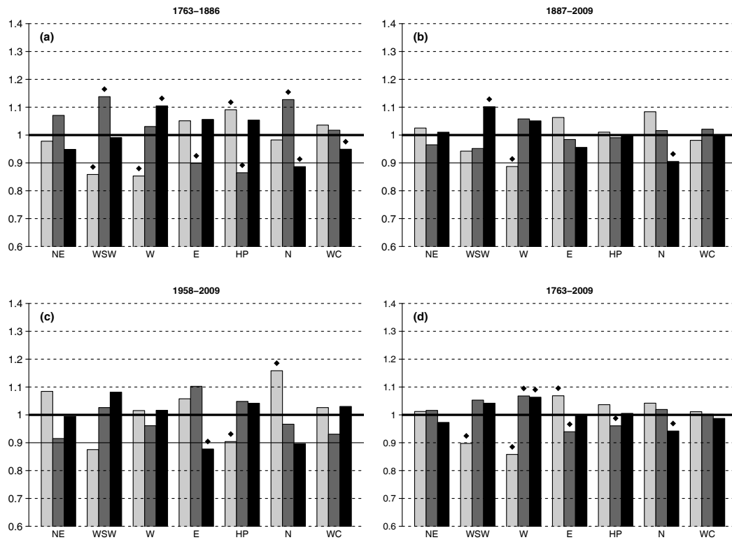
Figure 5. Ratios of the frequency for the low (light grey), moderate (grey), and high (black) solar activity classes relative to the long-term mean for different periods. Dots correspond to statistical significance of the ratios at the 95 % level.
