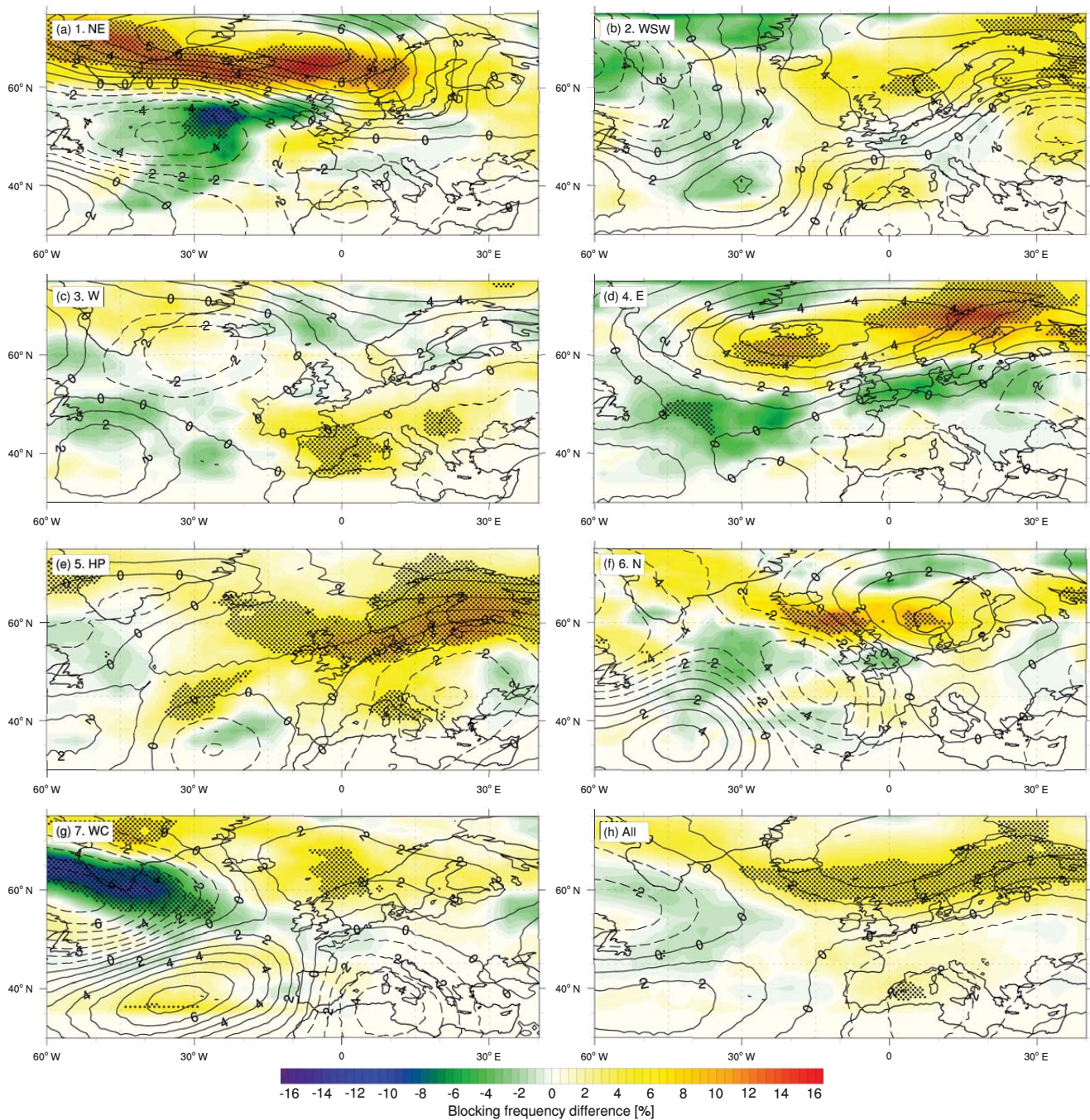
Figure 7. CAP7 (1 to 7) and mean (All) JFM blocking frequency (colour) in % and 500 hPa geopotential height (contour) in gpdm difference between low and high solar activity (low minus high) computed with ERA-40/Interim for the period 1958–2009. The 95 % significance level is indicated by stippled areas.
