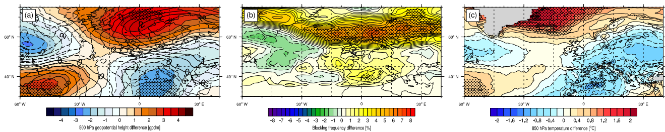
Figure 4. 1958–2009 low minus high solar activity differences computed with ERA-40/Interim. (a) 500 hPa geopotential height (colour) in gpdm and sea level pressure (contour) in hPa. (b) Blocking frequency in %. (c) 850 hPa temperature in °C. The 95 % significance level is indicated with stippled areas.
