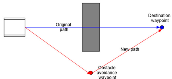
Figure 3. Obstacle avoidance algorithm schematic
