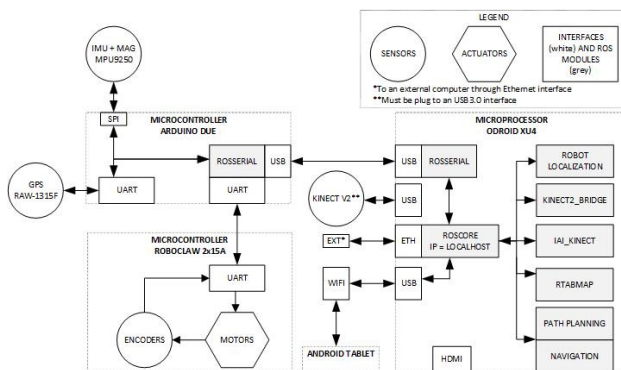
Figure 2. Schematic diagram
