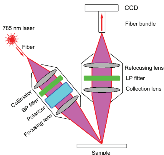
Figure 1 The configuration of the polarized Raman probe. Abbreviations: BP, band pass; CCD, charge-coupled device; LP, long pass.
