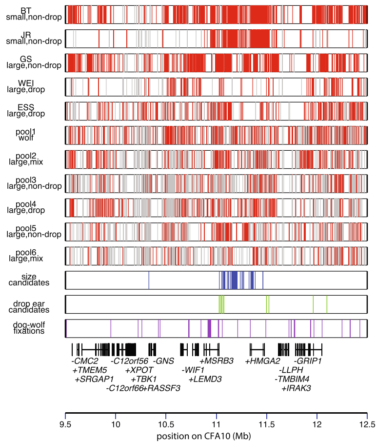
Fig. 2 Patterns of SNP variation in a 3 Mb region on CFA10. The first 5 bars show variation in the sequence capture (SC) pools of single breeds and the next 6 bars show variation in the whole genome sequencing pools (WGS; see Table 2 for details). Red lines represent SNP positions that are fixed for a non-reference allele in a particular pool, grey lines represent SNP positions that cannot be confidently assessed due to low coverage. Sites that are polymorphic within a breed, or that match the reference allele are not marked. The bottom 3 bars represent SNPs that display patterns of fixation that matches phenotypic variation. Candidate SNPs for controlling variation in body mass (blue) ear type (green) and those that are fixed for alternate alleles in all dogs compared to wolves (purple) are shown. The location of protein coding genes in the region are also shown, which were identified by mapping human RefSeq genes onto the canFam2.0 dog assembly. Genes are labelled +/- according to direction of transcription. Ear and body mass candidates are concentrated in a region between the MSRB3 and HMG2 genes, whereas a cluster of dog-wolf fixations is found within the MSRB3 gene
