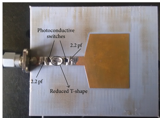
(c) Optically controlled filtenna
