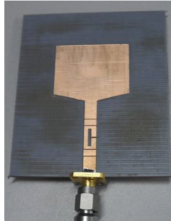
(b) The first filtenna prototype
