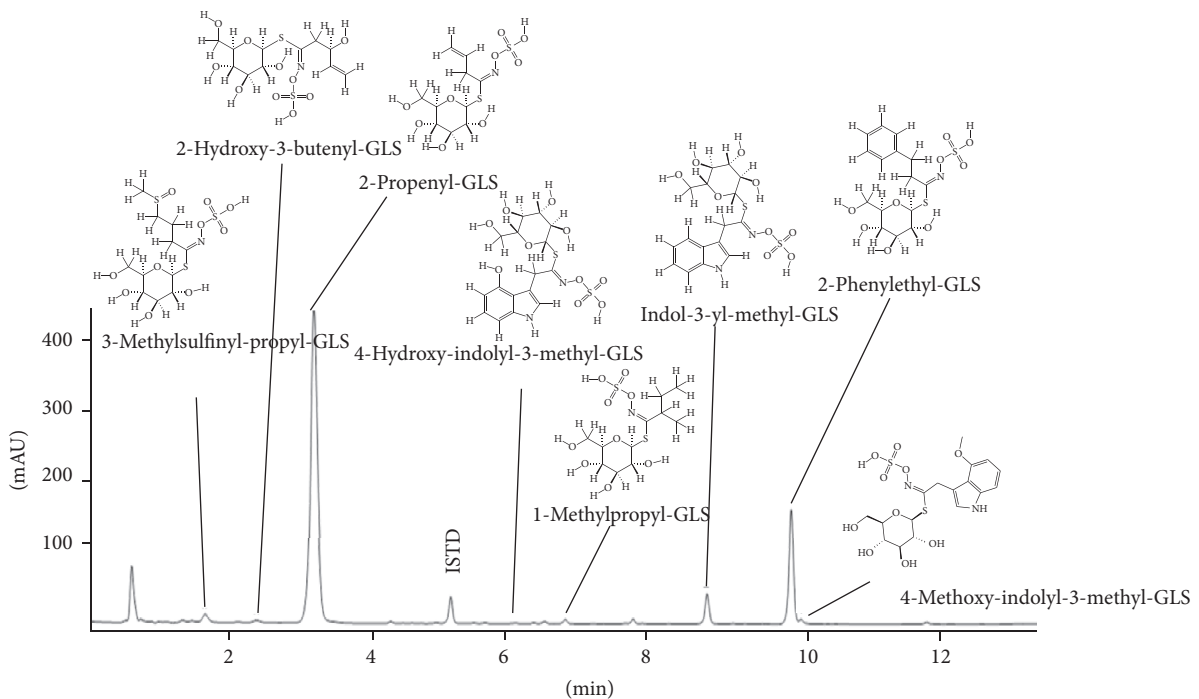
FIGURE 5: Glucosinolate profile of the aqueous extract of horseradish root. ISTD: internal standard; GLS: glucosinolate.
