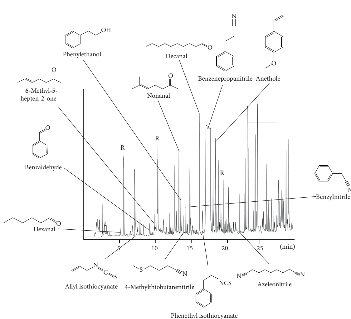
FIGURE 6: Nontargeted analysis of volatile compounds from the aqueous extract of horseradish root by GC-MS.
