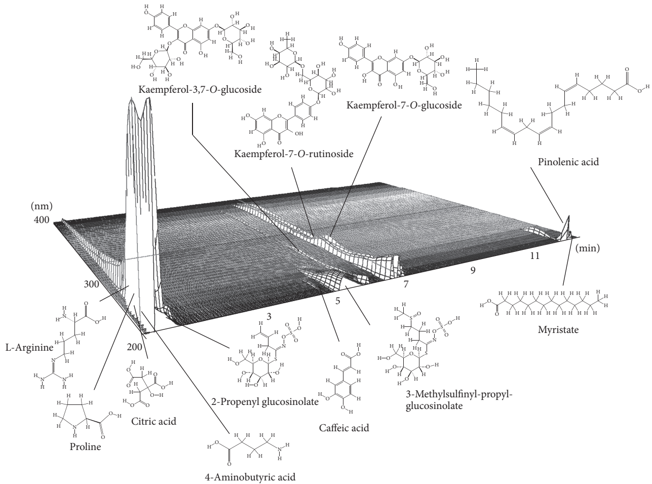
FIGURE 4: Metabolomic analysis of the aqueous plant extract using UHPLC-QToF-MS. The compounds were identified tentatively by comparing the mass spectra with MassHunter METLIN PCDL for the nonvolatile compounds and public available databases.
