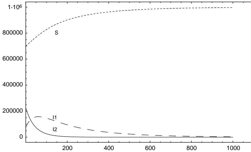
Figure 1. Shows the numerical simulation of our model and gives approximate results of the (S(t), I_1(t), I_2(t)) , when the basic reproductive numbers have the values (R_{01}, R_{02}) = (0.8, 0.6) .
