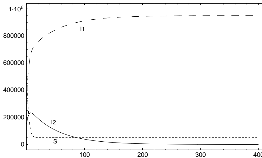
Figure 2. Shows the numerical simulation of our model and gives approximate results of the (S(t), I_1(t), I_2(t)) , when the basic reproductive numbers have the values (R_{01}, R_{02}) = (20.0, 10.0) .
