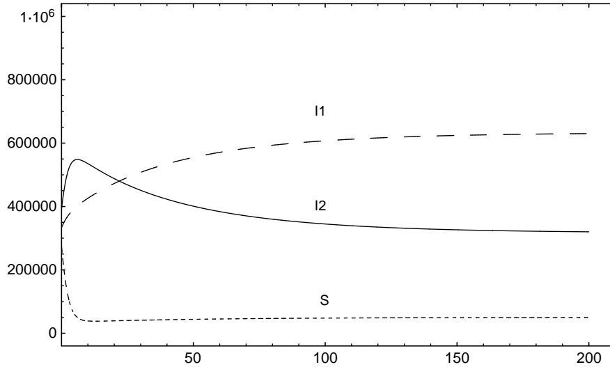
Figure 3. Shows the numerical simulation of our model and gives approximate results of the (S(t), I_1(t), I_2(t)) , when the basic reproductive numbers have the values (R_{01}, R_{02}) = (10.0, 20.0) .
