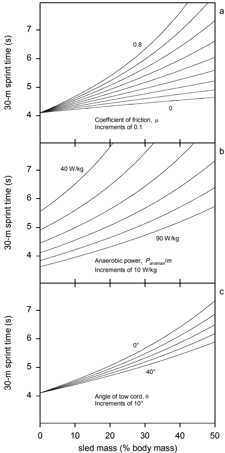
Fig. 4 These plots show the effects on an athlete's 30-m sprint time (when towing a weighted sled) of: (a) the coefficient of friction; (b) the athlete's anaerobic power; and (c) the angle of the tow cord. Calculations are for a standard athlete with P_{\text{anamax}}/m = 70 \text{ W/kg} , m =
