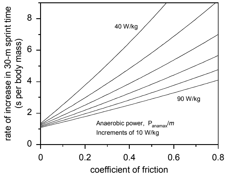
Fig. 5 This plot shows the effect of the coefficient of friction of the running surface ( \mu ) on the rate of increase in 30-m sprint time (for a sled mass of less than about 10% of body mass). Calculations are for a standard athlete. These results indicate that we should expect to see greater inter-athlete differences in the rate of increase in sprint times on a running surface with a higher coefficient of friction
