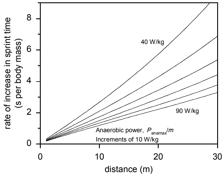
Fig. 6 This plot shows the effect of sprint distance on the rate of increase in sprint time (when the sled mass is less than about 10% of body mass). Calculations are for a standard athlete with \mu = 0.6 . These results indicate that we should expect to see greater inter-athlete differences in the rate of increase in sprint times when timing athletes over a longer distance
