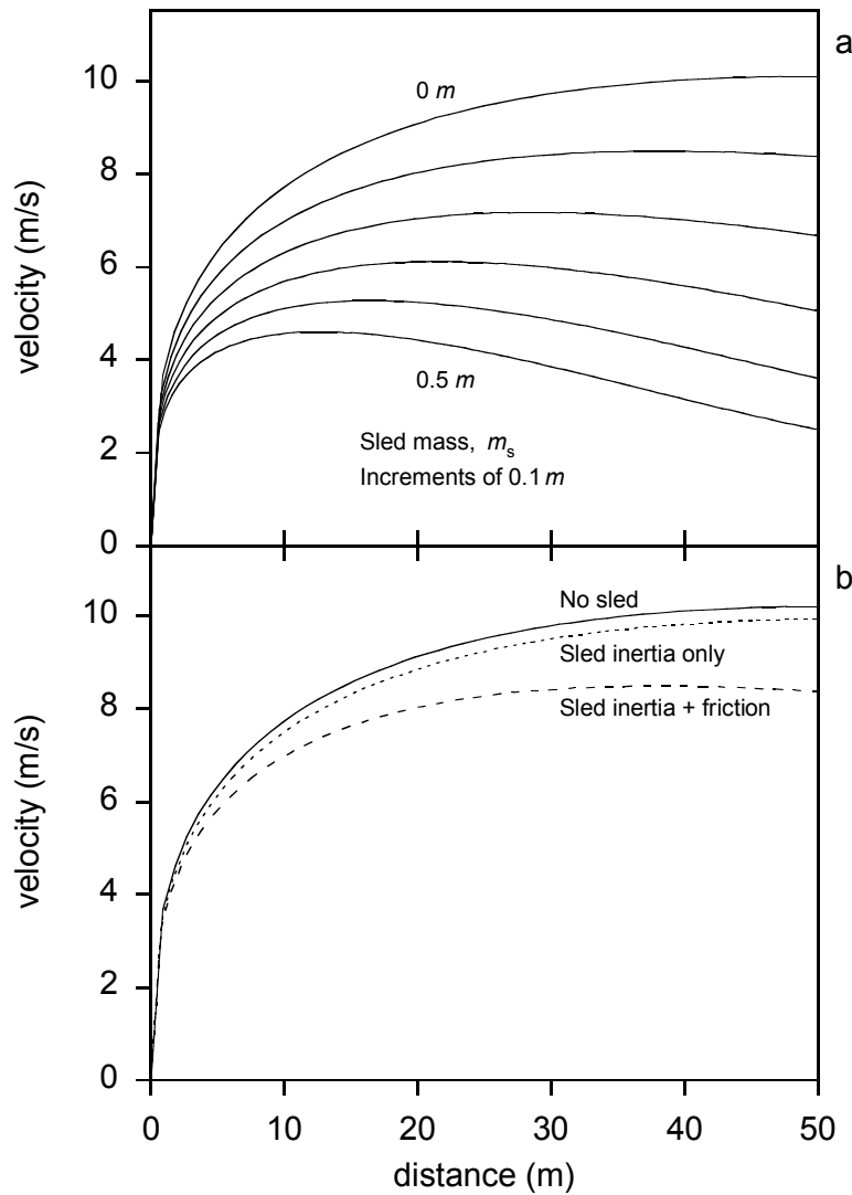
Fig. 2 Plot (a) shows the effect of the mass of the sled ( m_s ) on an athlete's velocity profile when towing a weighted sled. Calculations are for a standard athlete with P_{\text{anamax}}/m = 70 W/kg, m = 70 kg, \mu = 0.6 , and \theta = 0^\circ . The main effects of a heavier sled are to reduce the maximum velocity attained by the athlete and to reduce the distance at which the athlete begins to slow down. Plot (b) shows the relative contributions of sled inertia and sled friction to the athlete's velocity profile: no sled (solid line); sled inertia only (short-dash line); and sled inertia and sled friction (long-dash line). Calculations are for a standard athlete with P_{\text{anamax}}/m = 70 W/kg, m = 70 kg, m_s/m = 0.1 , \mu = 0.6 , and \theta = 0^\circ . In a sled-towing exercise
