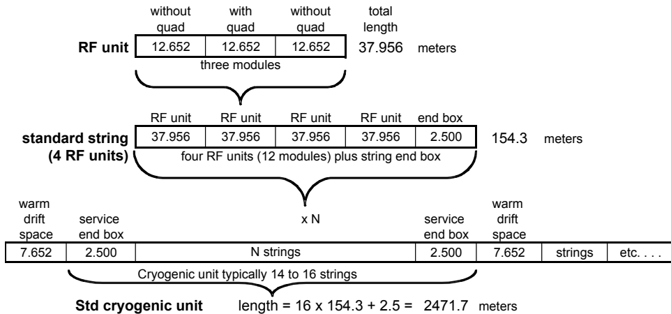
FIGURE 3. Division of main linac into cryogenic strings
