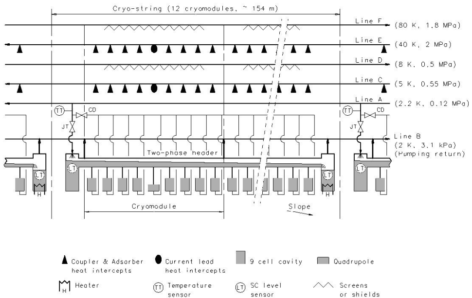
FIGURE 2. ILC main linac cryogenic string
