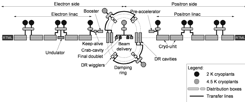
FIGURE 1. The overall layout concept for the cryogenic systems.
