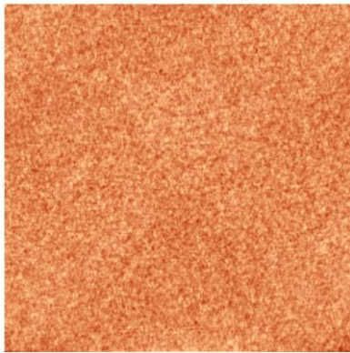
Fig. 7 – 10 × 10 μm AFM image of p-n structure surface after growth
