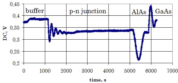
Fig. 6 – Detector voltage versus growth time dependance for p-n structure growth
