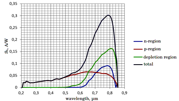
Fig. 4 – Calculated spectral response of p-i-n GaAs structure
