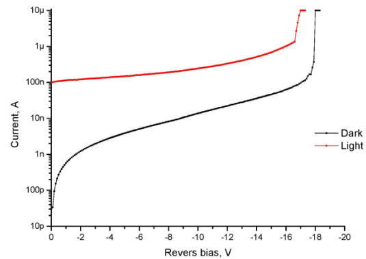
Fig. 8 – I-V measurements of fabricated p-n photodiode
