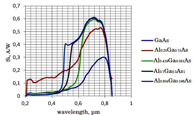
Fig. 5 – Calculated spectral response of p-i-n AlGaAs heterostructure with different mole fraction of Al
