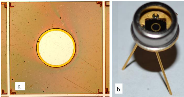
Fig. 2 – 4 × 4 mm chip with active region 1.5 mm in diameter (a) and packed chip (b) of p-n photodetector
