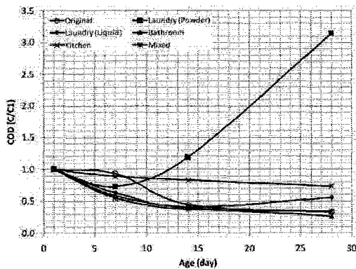
Fig. 11: COD vs. time.
