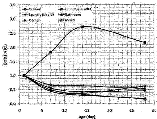
Fig. 12: BOD vs. time.
