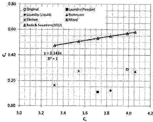
Fig. 3: C_s - C_c plots.
