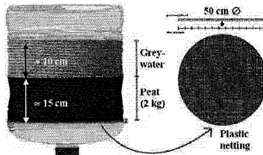
Fig. 1: Test setup of the greywater filtration system.
