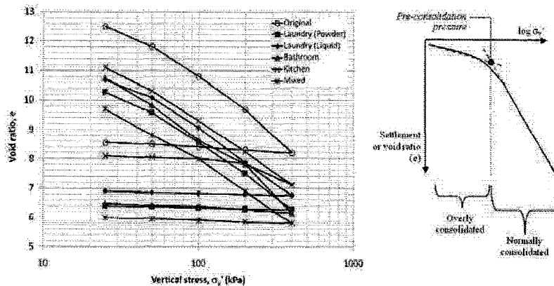
Fig. 2: Compression curves of peat specimens (post-filtration)
