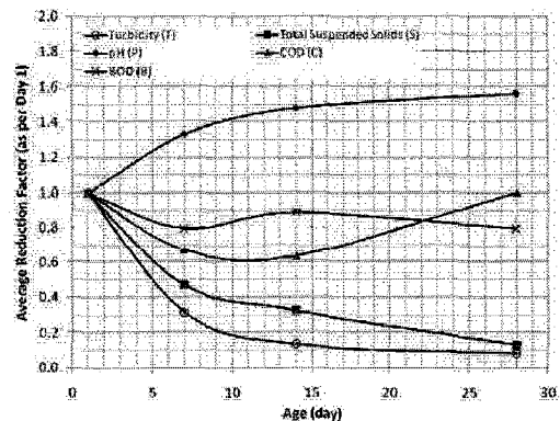
Fig. 13: Average Reduction Factor vs. time
