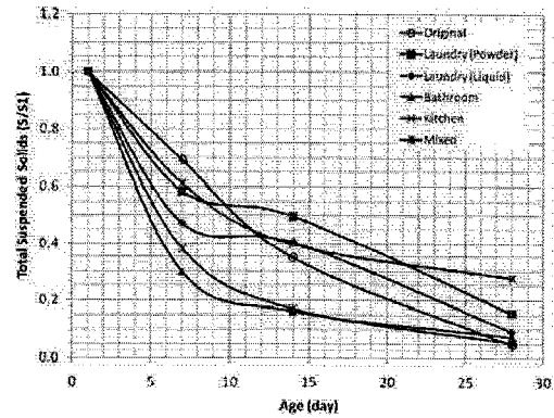
Fig. 9: Total Suspended Solids vs. time.
