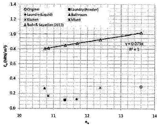
Fig. 4: C_s - e_0 plots.
