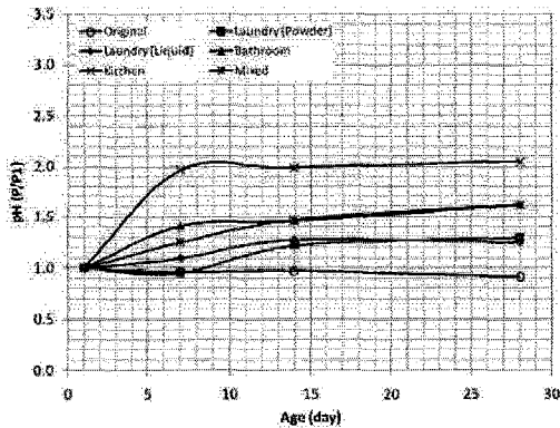
Fig. 10: pH vs. time.
