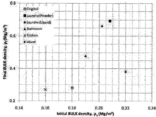
Fig. 7a: Bulk densities, \rho_r - \rho_o plots
