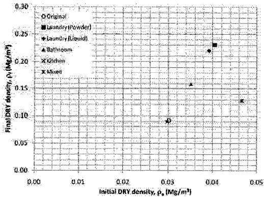
Fig. 7b: Dry densities, \rho_r - \rho_o plots
