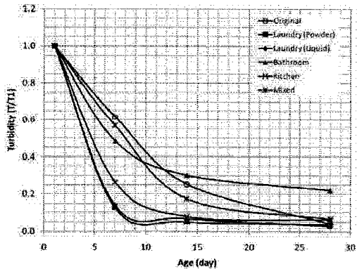
Fig. 8: Turbidity vs. time.
