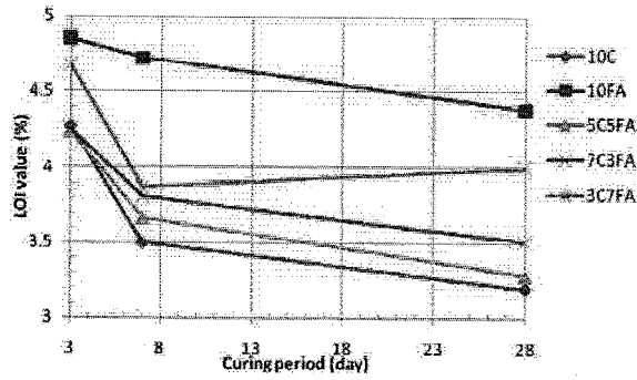
Fig. 6: LOI values at different curing times
