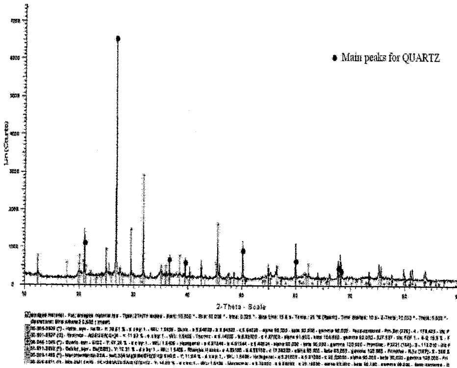
Fig. 8: XRD analysis of the dredged sample
