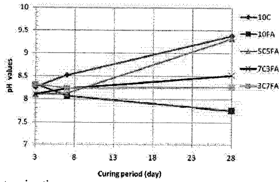
Fig. 7: pH readings at different curing times
