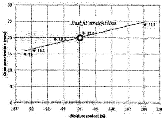
Fig. 2: Cone penetration versus moisture content
