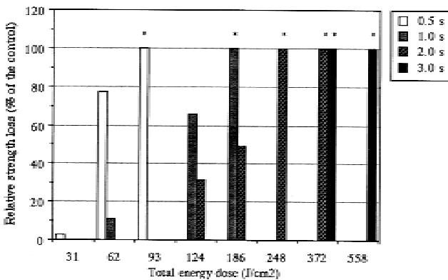
Fig. 2. Relative strength loss of the nylon suture at identical total light doses at different pulse durations. An asterisk (*) signifies that the thread disrupted during irradiation (100% loss of strength).
