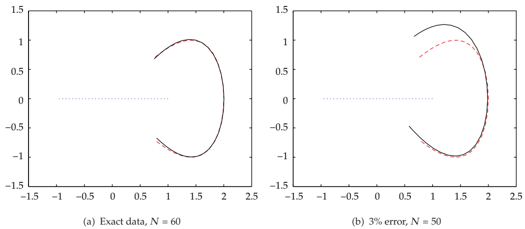
Figure 6: d \pm \pi/4 .
