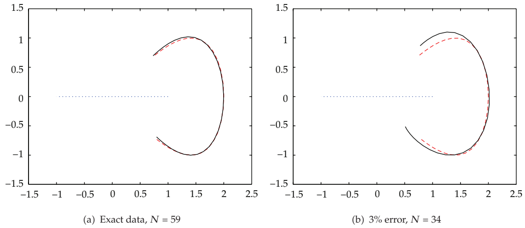
Figure 5: d \pm \pi/2 .
