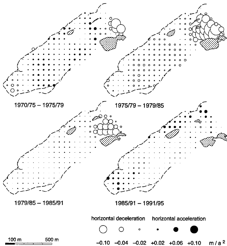
Figure 12 Changes in horizontal surface velocity with time, Gruben rock glacier.
