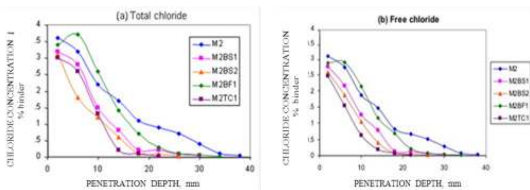
Figure 6 Chloride profiles for concrete at water-to-binder ratio of 0.35 under sodium chloride solution
