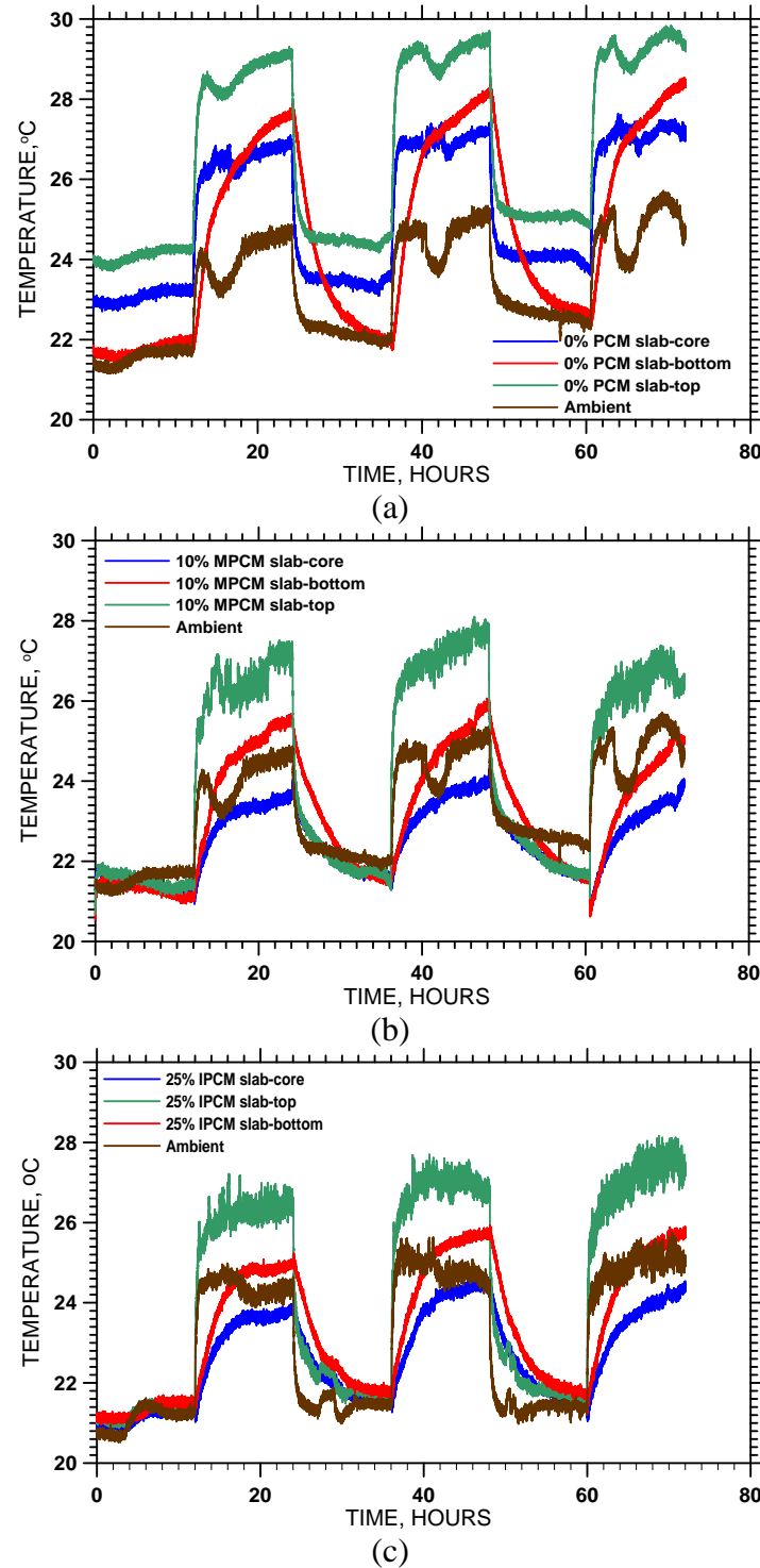
Figure 11 Temperature studies during 72 hours day and night cycles of (a) Plain mortar slab, (b) 10% MPCM modified slab and, (c) 25% IPCM modified slab
