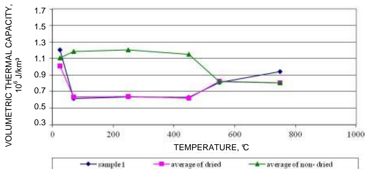
Figure 13 Volumetric thermal capacity dependence on temperature – FIREBOARD
