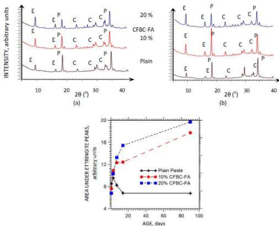
Figure 10 (a) and (b) XRD patterns of plain paste, 10%, and 20% CFBC fly ash modified pastes at 14 and 90 days respectively (E-Ettringite, C-Calcite ( \text{CaCO}_3 ), P-Portlandite ( \text{CH} )), (c) Estimated amounts of ettringite for plain, 10% and 20% CFBC fly ash modified pastes up to 90 days of curing.
