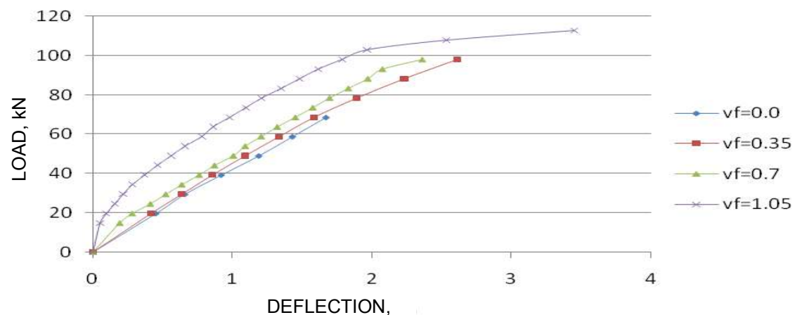
Figure 9 Load-deflection relationships for beams with a_v/d of 2.69
