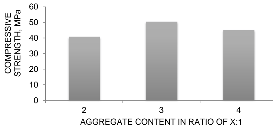
Figure 6 Comparison of the one-hour test results of the three different aggregate contents; with corresponding compressive strength at one hour.
