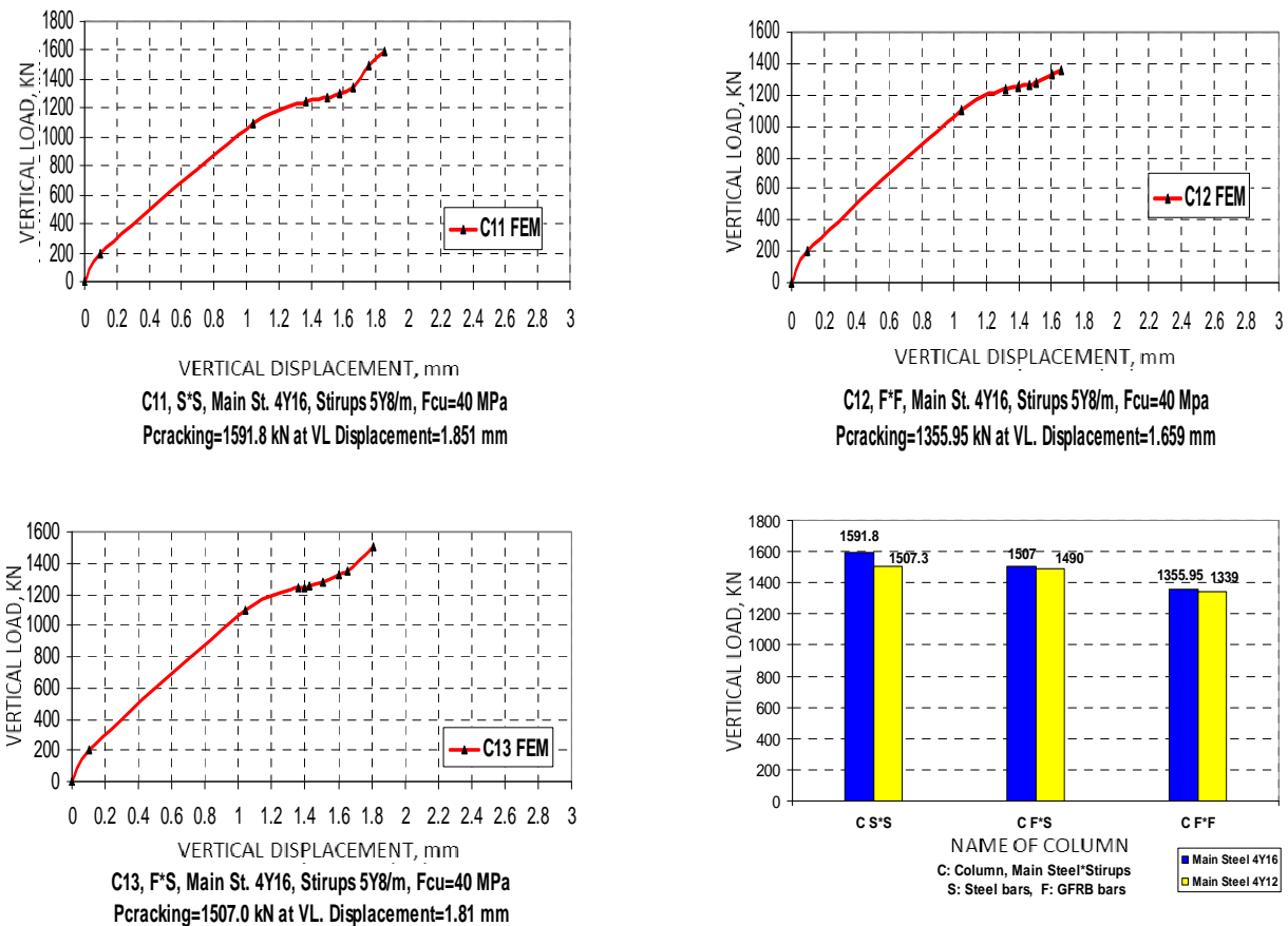
Figure 11 Effect of change the area of main steel.
