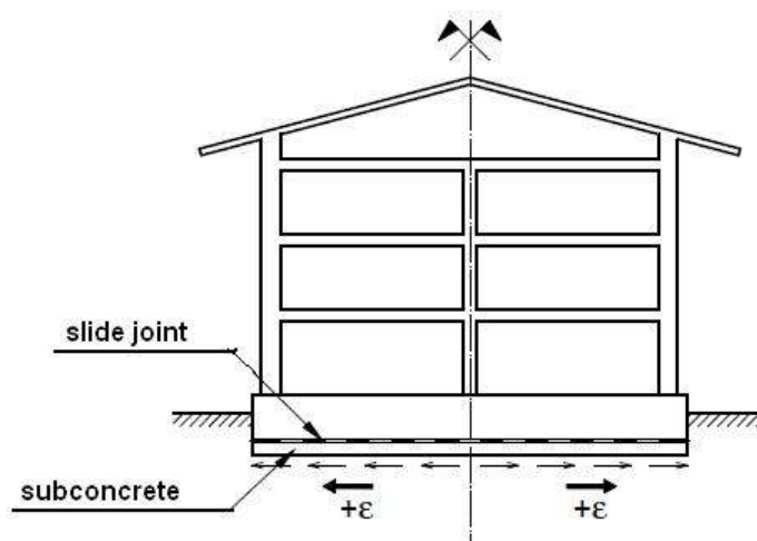
Figure 1 Schematic drawing of sliding joint
