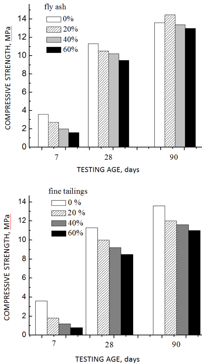
Figure 5 Compressive strength of 1000kg/m 3 mixtures as a function of time
