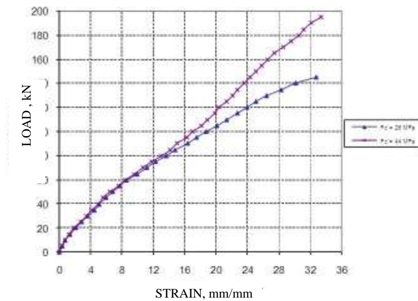
Figure 6 Effect of compression resistance on the relationship between load and strain for steel reinforced samples
