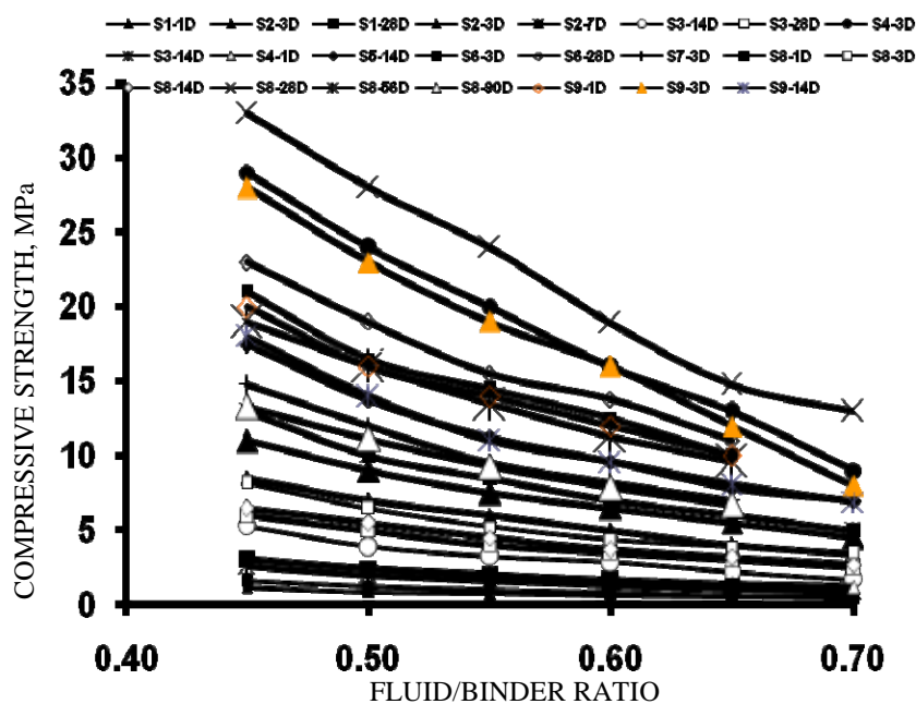
Figure 6 Variation of compressive strength verses f/b ratio (Abrams' Law)
