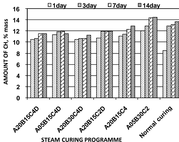
Figure 6 Effects of steam curing on amount of CH generated
