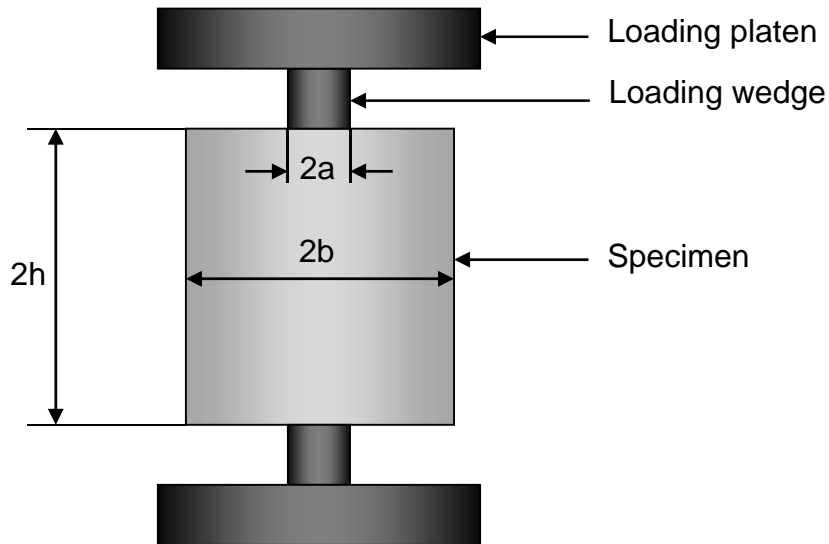
Figure 1 Geometry of the layout of Barcelona test
