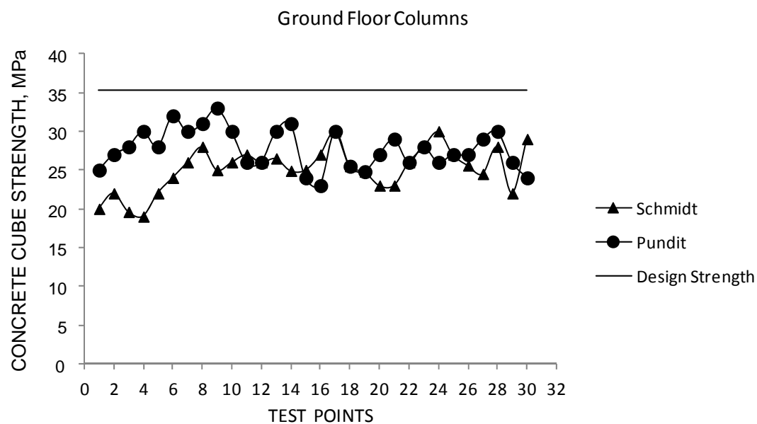
Figure 11 Comparison between nondestructive cubic strength and design strength
