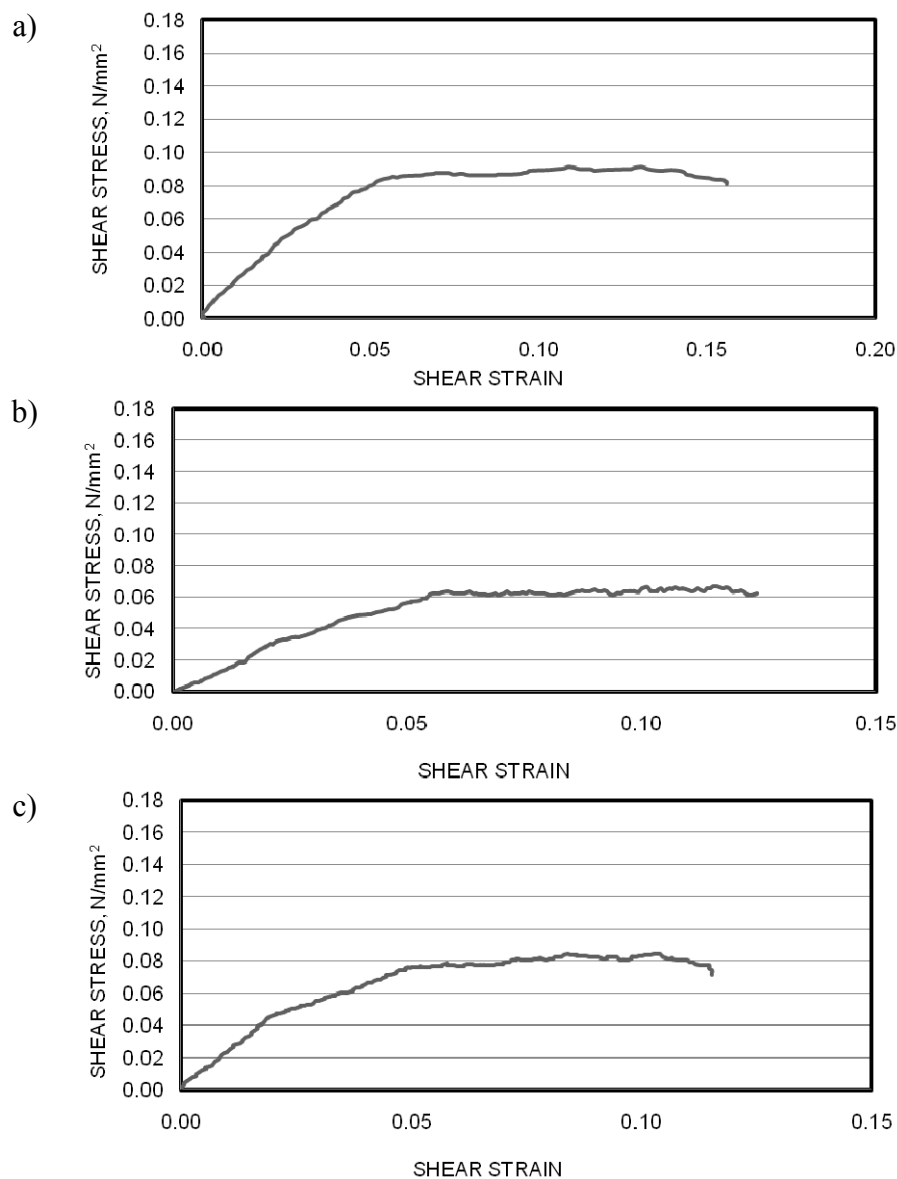
Figure 2(a, b, c) Shear stress versus shear strain curves for mix G at normal stress of 0.015 N/mm 2 and displacement rates of (a) 5 mm/min, (b) 15 mm/min and (c) 25 mm/min
