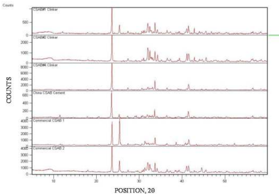
Figure 1 XRD profiles of the laboratory synthesized clinkers compared to the commercially available CSAB cements. K = Klein's Compound; An = anhydrite; B = belite (C 2 S).
