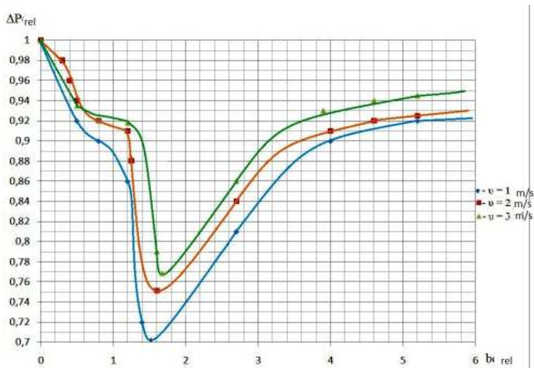
Figure 10 Influence of a relative thickness of adsorption molecular layers of "Efren 1" on a hydraulic resistance of the pipeline
