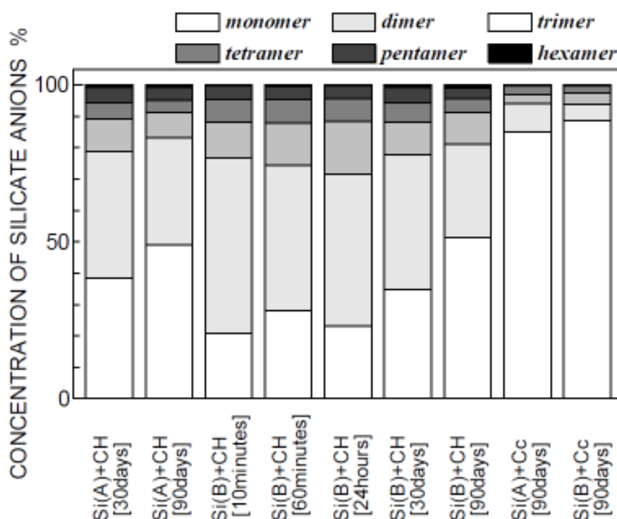
Figure 10 Polymer ratio of silicate anion in hardened specimen treated with alkaline silicate solution vs. hydration time
