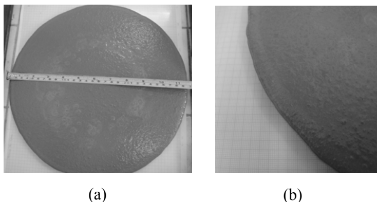
Figure 5 Testing with truncated cone showing (a) the final spread and (b) non-segregation of the mortar
