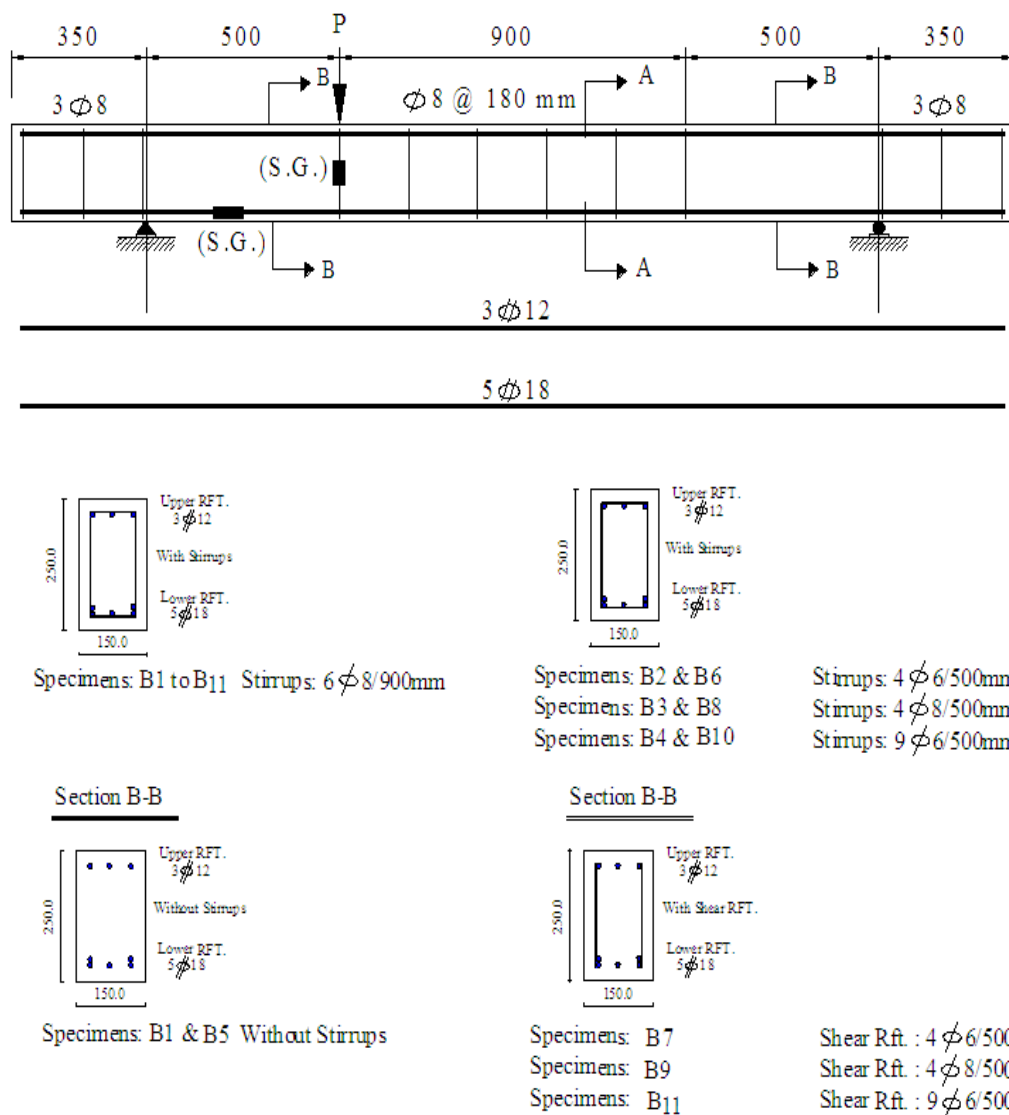
Figure 2 Test set up, Details of Reinforcement, and Strain Gauge for Tested Beams
