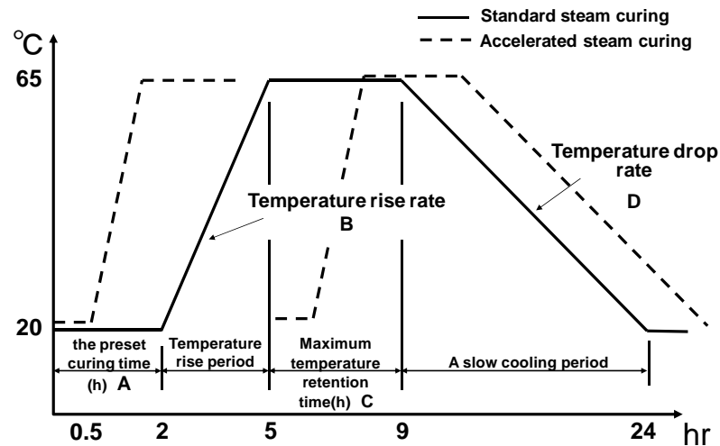
Figure 1 Steam curing program
