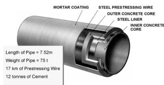
Figure 2 Cross section of pipe
