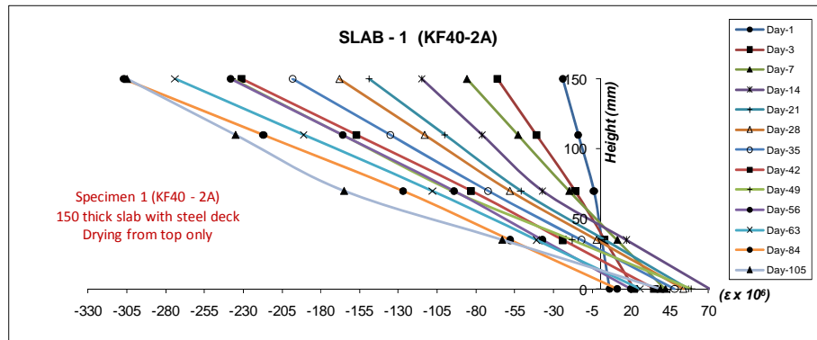
(a) Specimen - KF40-A – 150 mm thick slab with steel decking in place
