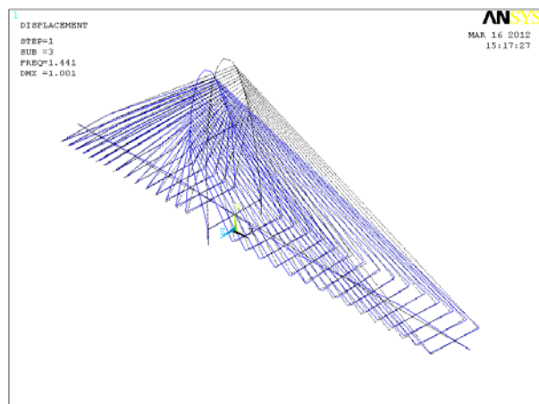
Figure 1 The nodes of the whole bridge Figure 2 The model with 3 order vibration mode
