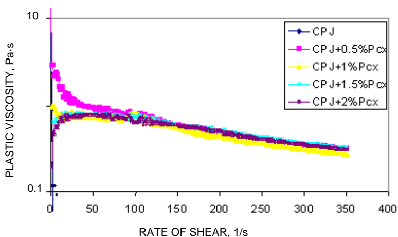
Figure 4 Plastic viscosity according to the rate of shear for a CPJ without and with various percentages of Polycarboxylate with W/C = 0.35
