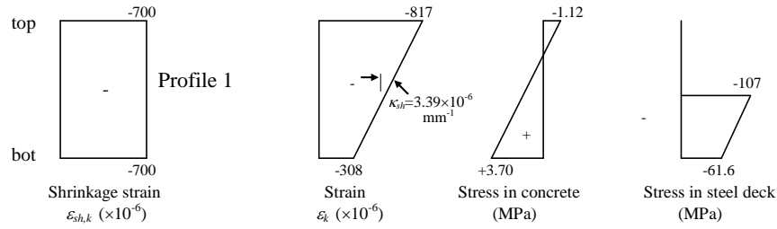
(b) Uniform shrinkage profile ( \epsilon_{sh,k} = -700 \times 10^{-6} top and bottom)
