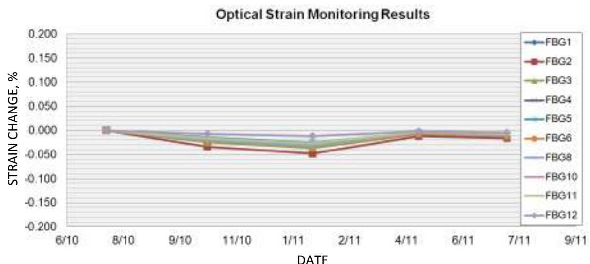
Figure 9 Changes in strains over the monitoring period
