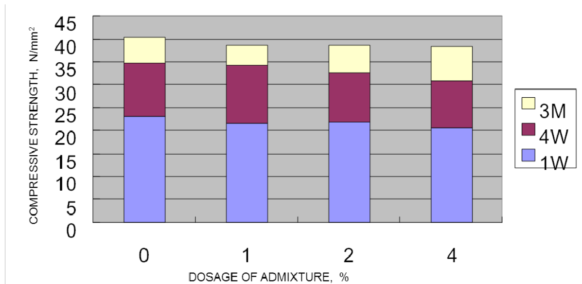
Figure 1 Compressive strength (w/c 60%, sl 18cm)
