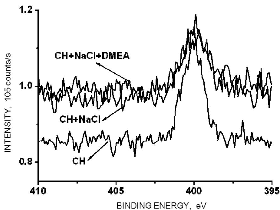
Figure 5 \text{N}1s spectra of steel surface in different environment
