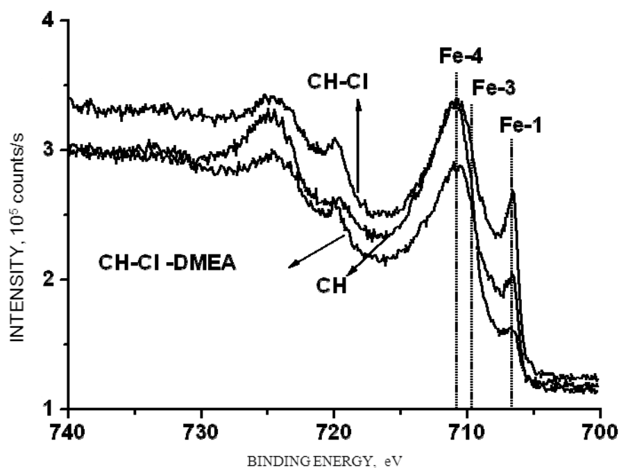
Figure 4 \text{Fe}_{2p} spectra of steel surface in different environment
