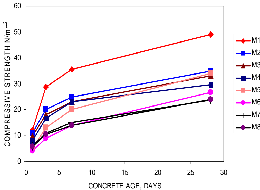
Figure 3 Compressive strength developments of concretes
