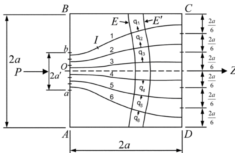
Figure 1 Dispersion of compression provided by Guyon [1]
