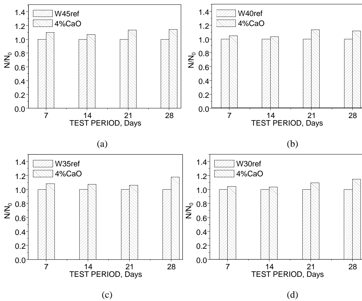
Figure 7 Quantity of dissolved \text{Ca}^{2+}
