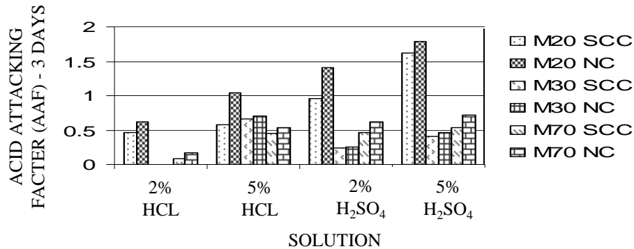
Figure 4 Acid Attacking Factors for SCC and NC at the 3 days of immersion
