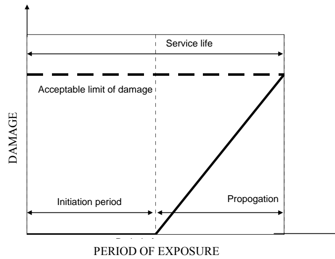
Figure 3 Traditional model for corrosion
