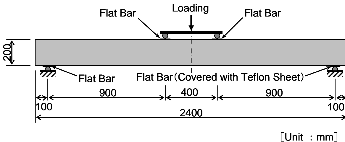
Figure 4 Experimental method
