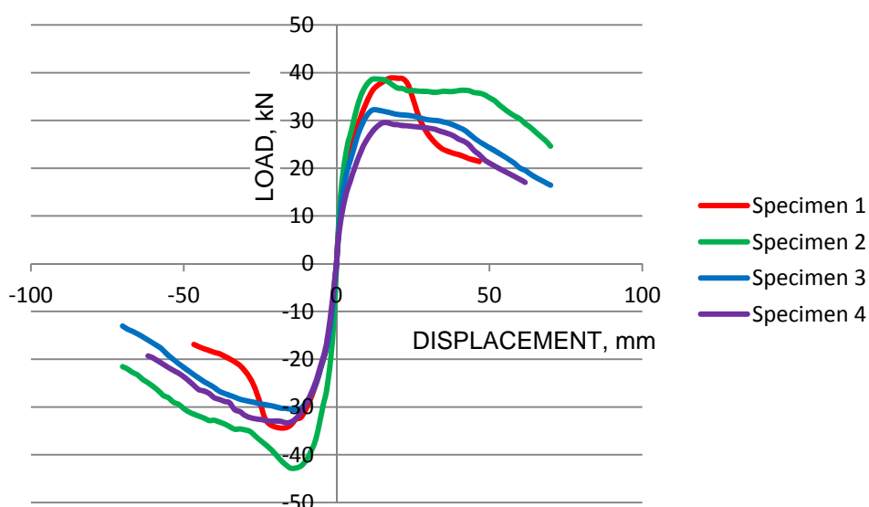
Figure 9 Envelope curves for hysteresis loops
