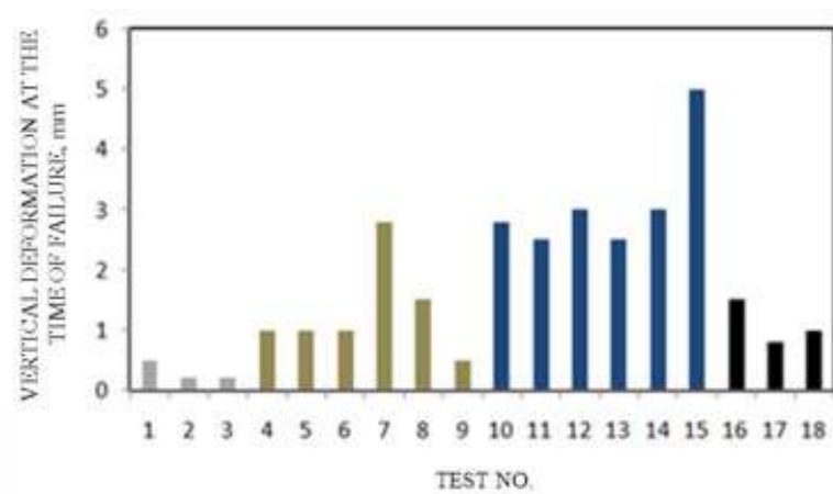
Figure 15 Summary of vertical deformations at the time of failure
