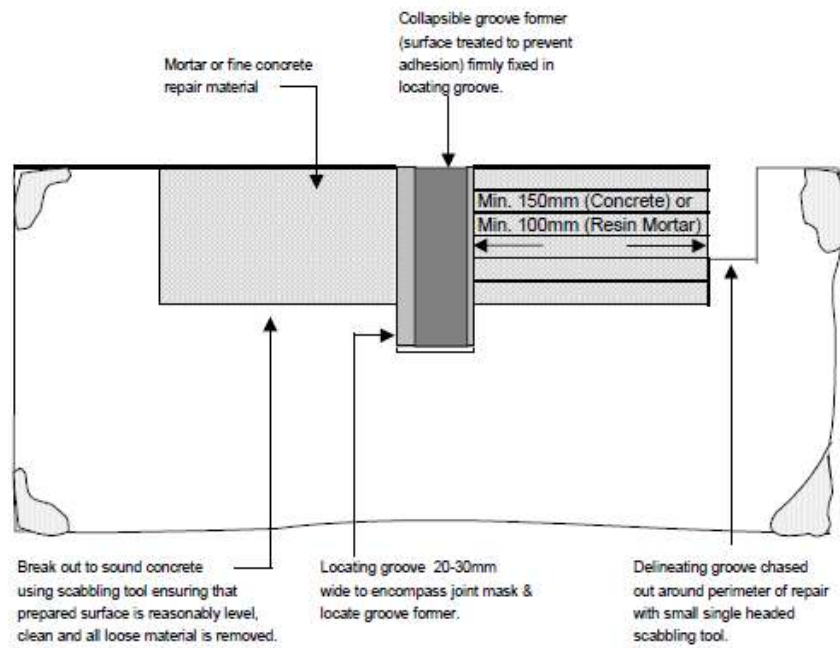
Figure 1 Typical situation on concrete road repair
