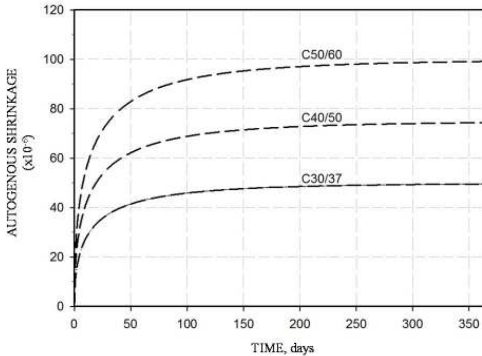
Figure 3 Autogenous shrinkage curves (reproduced from Eurocode 2 [2])
