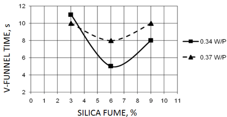
Figure 3 Effect of silica fume on V-Funnel Index
