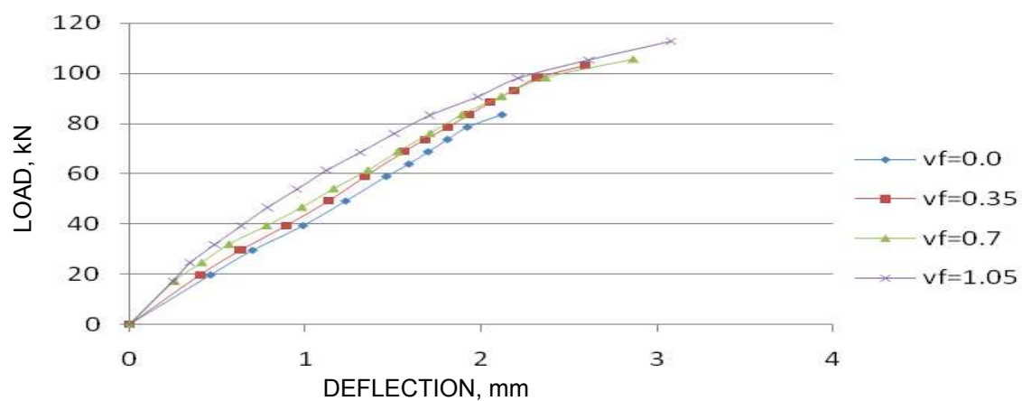
Figure 8 Load-deflection relationships for beams with a_v/d of 2.46
