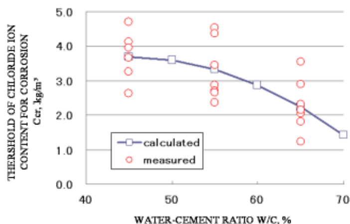
Figure 3 Threshold of chloride ion and water-cement ratio (○ indicates experimental data.)
