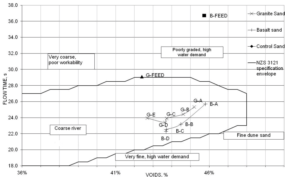
Figure 2 New Zealand Flow Cone results and specification envelope
