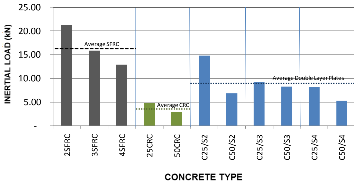
Figure 4 Inertial Load
