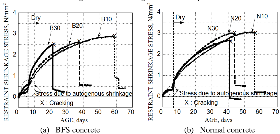
Figure 5 Free shrinkage test result examples
