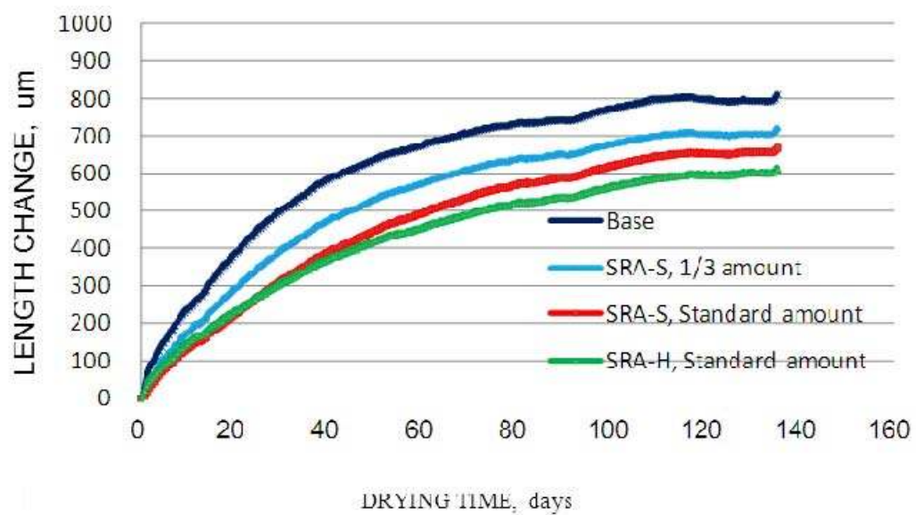
Figure 3 Drying shrinkage
