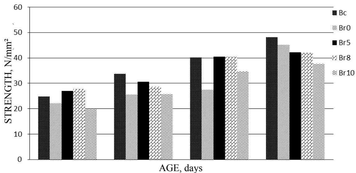
Figure 3 The compressive strength development (Rc) as a function of concrete age for recycled and normal concrete
