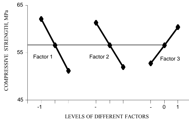
Figure 6 Response of different factors on compressive strength
