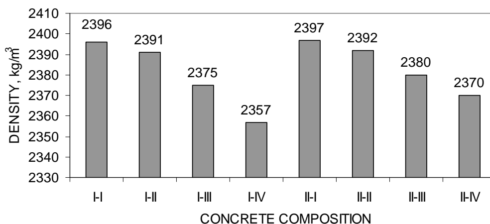
Figure 5 Concrete densities
