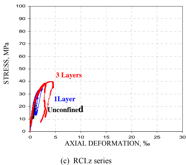
Figure 2 Stress strain curves of NSC CFRP confined specimens
