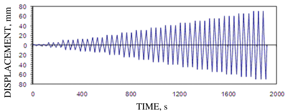
Figure 5 Displacement history
