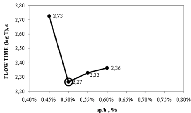
Figure 4 Marsh cone curve detailing the saturation point of the superplasticizer
