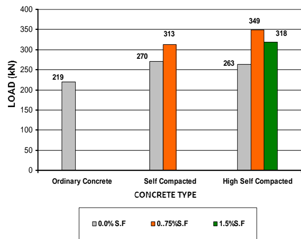
Figure 8 Punching shear forces for all the tested specimens
