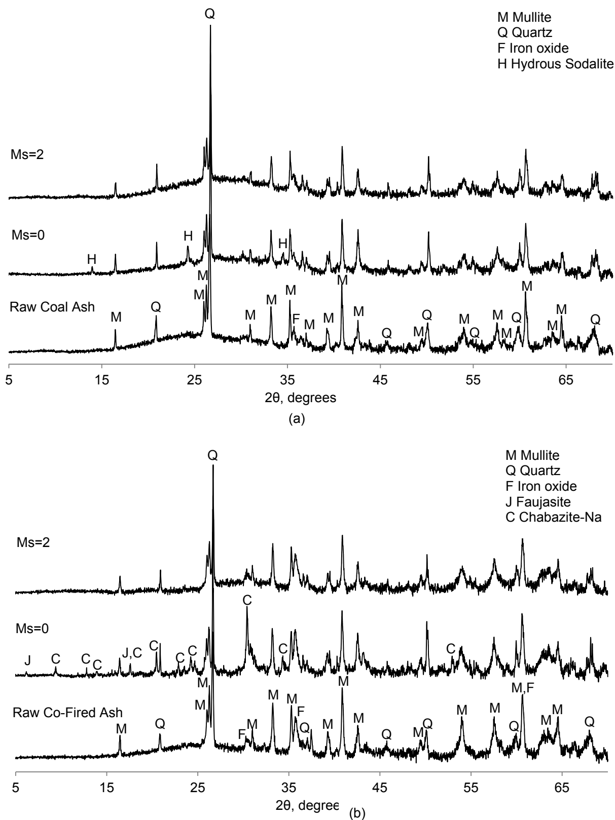
Figure 2 X-ray diffraction patterns of (a) coal ash sodium-activated pastes and (b) co-fired ash sodium-activated pastes
