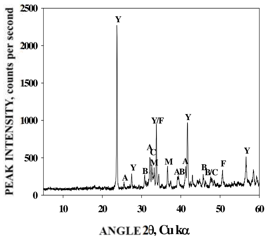
Figure 3 XRD pattern of mixture O at 1300°C: Y = C_4A_3\bar{S} , A = C\bar{S} , B = C_2S , C = C_3A , F = C_4AF , M = C_{12}A_7
