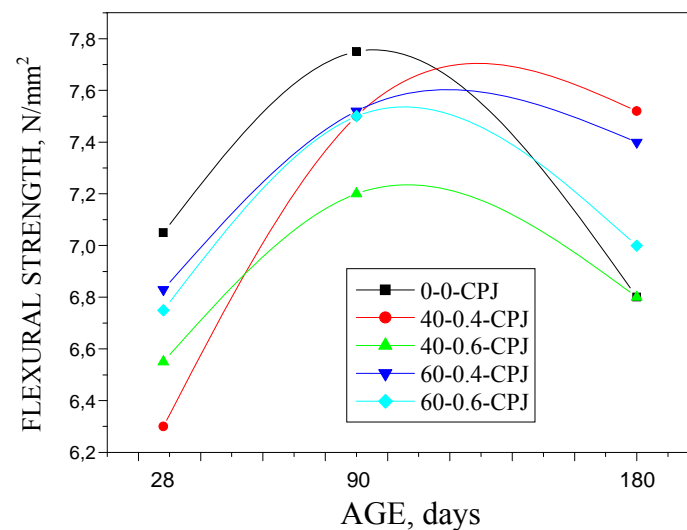
Figure 4 Flexural strength
