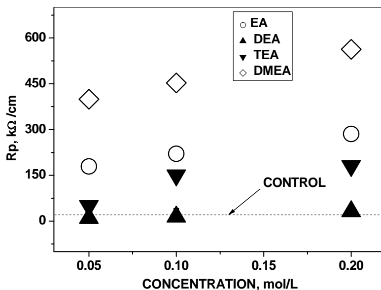
Figure 1 Inhibition effect of the studied amino alcohols (0.1mol/L Cl - )
