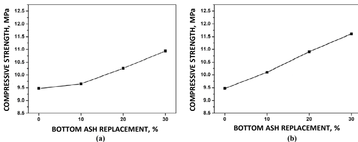
Figure 4 Compressive strength results at (a) FLWC and (b) BLWC
