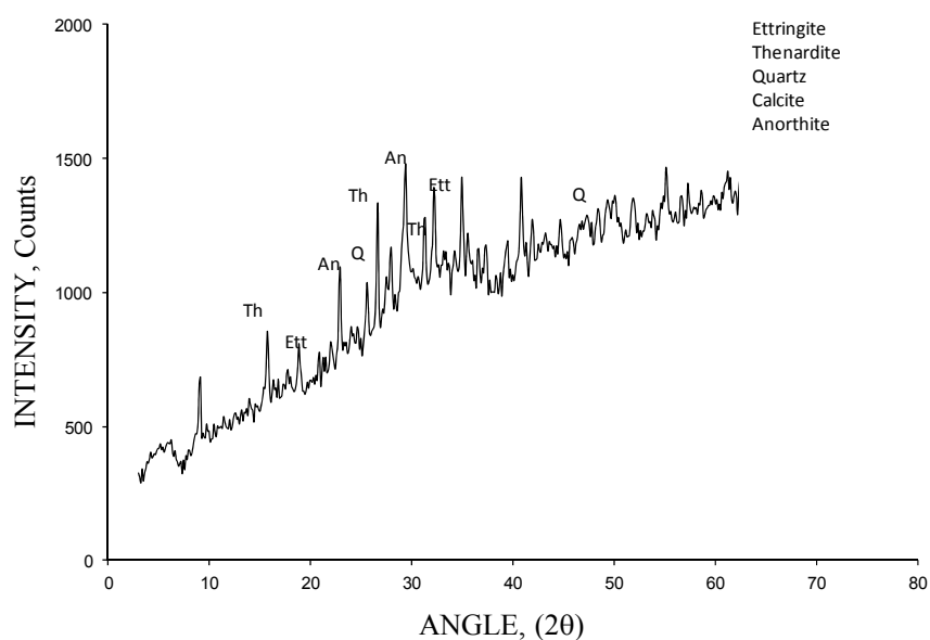
Figure 7 XRD diagram for HCFA paste geopolymerized in 40 °C, at 65%RH, at 28-d age
