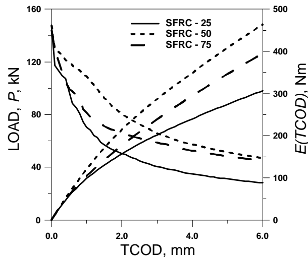
Figure 5 Post cracking response of FRC and energy determined by BCN test
