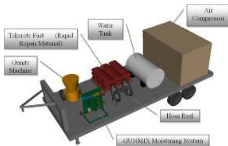
Figure 11 Conceptual drawing of the prototype delivery vehicle.
