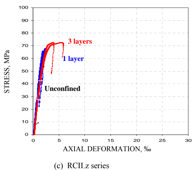
Figure 3 Stress strain curves of HSC CFRP confined specimens
