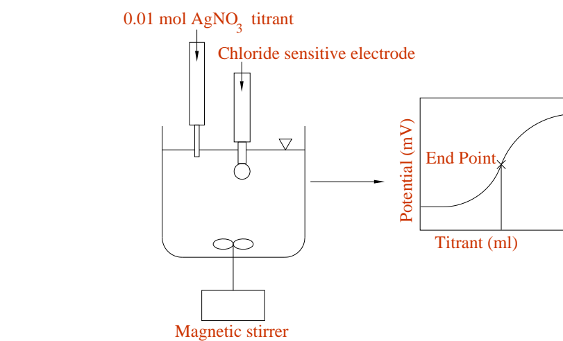
Figure 4 Working principle of Auto-titrator
