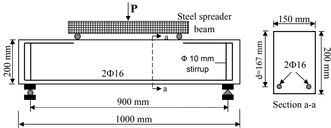
Figure 2 Details of the tested beams
