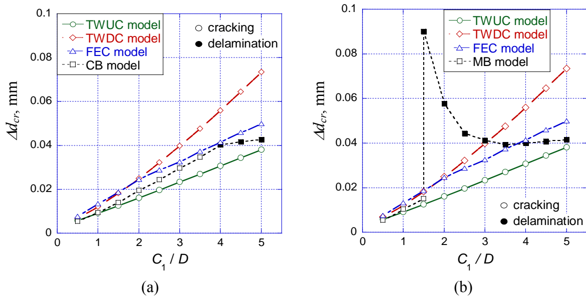
Figure 4 Comparison between the analytical models and the FE analysis (a) CB case; (b) MB case
