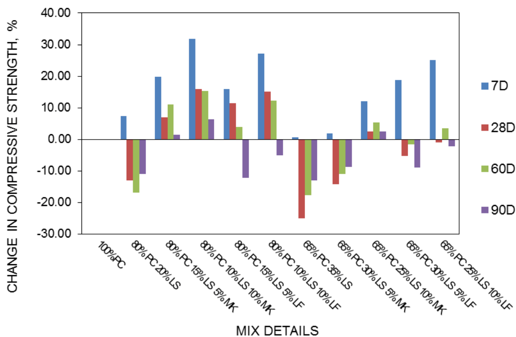
Figure 2 Normalized compressive strengths of concrete mixes w.r.t. control mix at 7 day curing age
