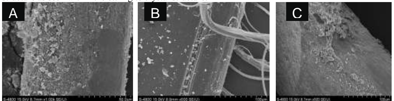
Figure 13 SEM images of fibres pulled from the OPC matrix: (A) PVA (1000x magnification); (B) PP (500x mag); (C) Steel (500x mag)
