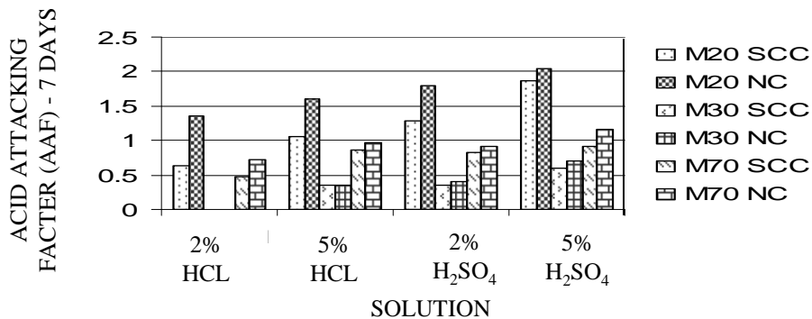
Figure 5 Acid Attacking Factors for SCC and NC at the 7 days of immersion
