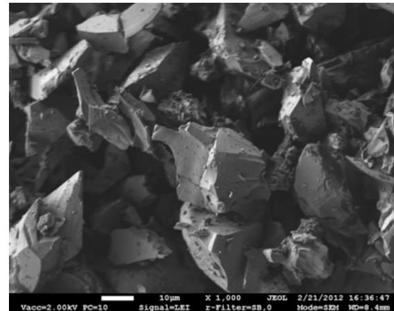
Figure 4 SEM micrograph of LB powder
