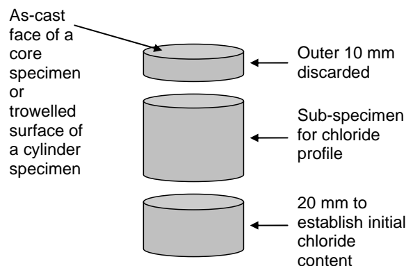
Figure 5 Specimen for determination of chloride diffusion coefficient
