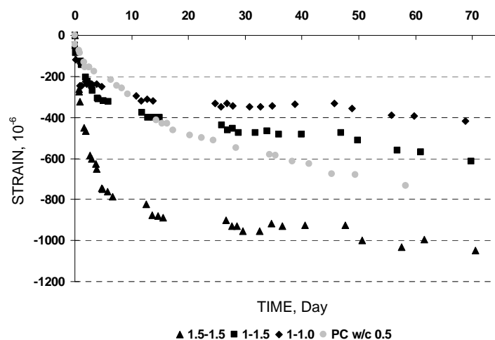
Figure 2 Drying shrinkage of AAF mortar and OPC w/c of 0.5 with time
