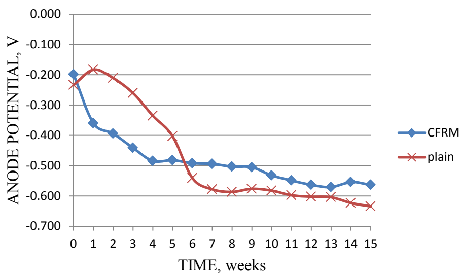
Figure 6 Corrosion potential of the anode bar with respect to a SCE
