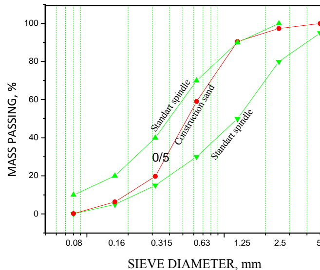
Figure 1 Sand curve
