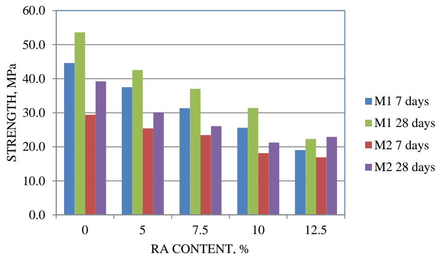
Figure 11 Compressive Strength vs rubber aggregate content
