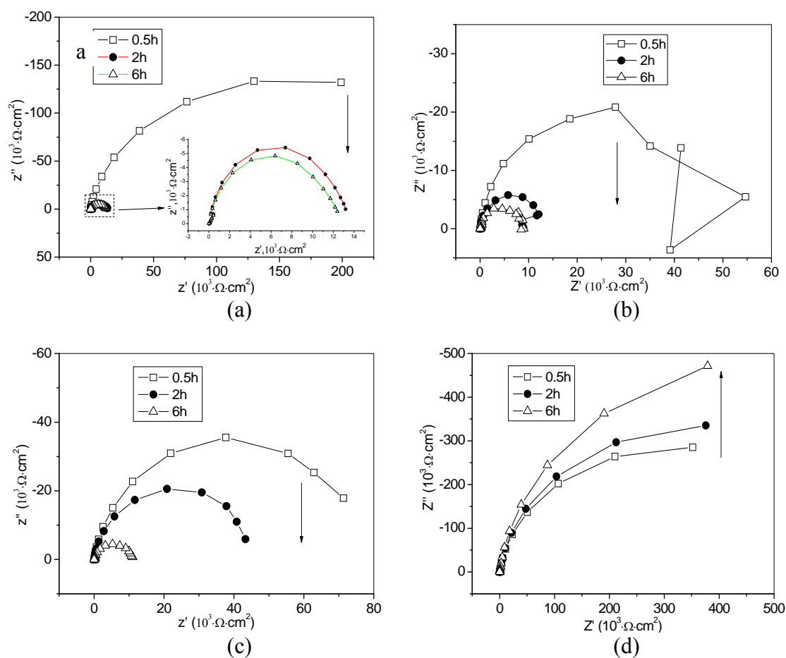
Figure 3 Transformation of inhibition effect with immersion time in SPS with 0.1mol/L \text{Cl}^- : (a) EA; (b) DEA; (c) TEA; (d) DMEA
