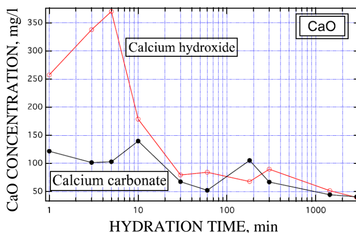
Figure 8 Solubility of calcium hydroxide or calcium carbonate in alkaline silicate solution with reaction time
