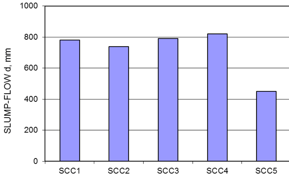
Figure 4 Slump-flow for the different mixtures prepared
