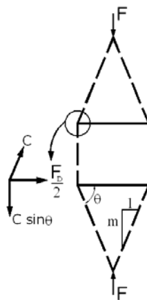
Figure 5 Equilibrium of simplified bottle-shaped strut
