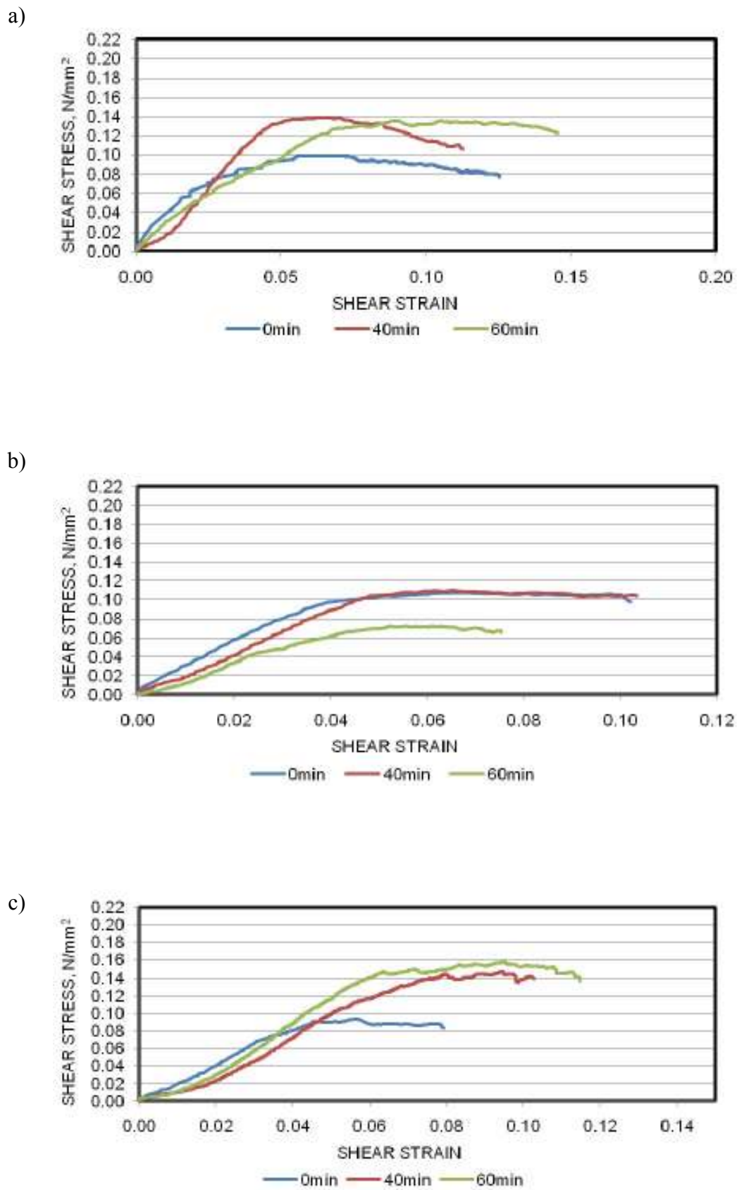
Figure 5(a, b, c) Shear stress versus shear strain curves for mix D at normal stress of 0.015 \text{ N/mm}^2 and displacement rates of (a) 5 \text{ mm/min} , (b) 15 \text{ mm/min} and (c) 25 \text{ mm/min}
