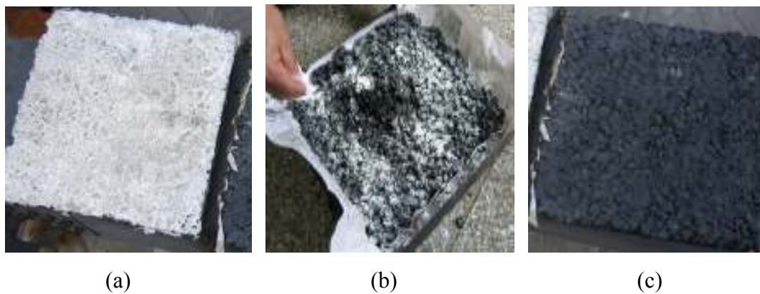
Figure 3 Three Ways of Adding Nano Titanium Dioxide
