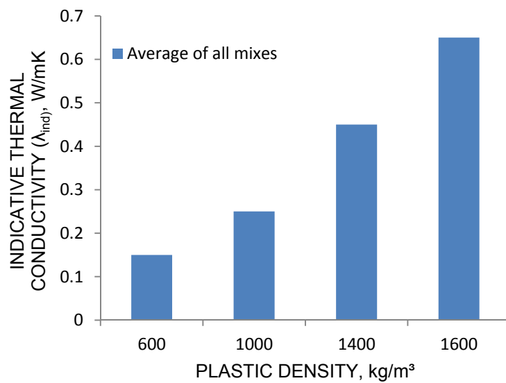
Figure 3 Effect of plastic density on indicative thermal conductivity of foamed concrete [6]
