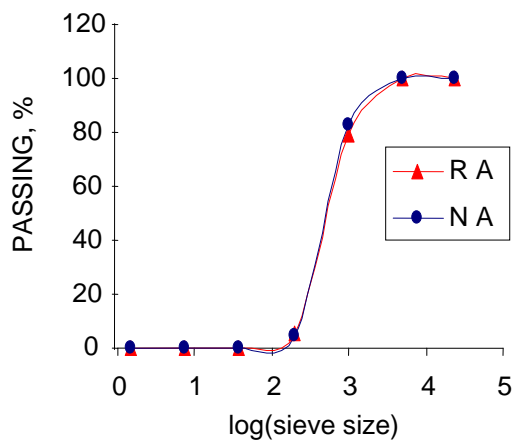
Figure 1 Percentage passing vs. logarithm of sieve size
