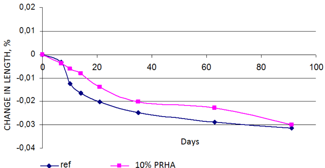
Figure 6 Shrinkage in concretes with and without PRHA
