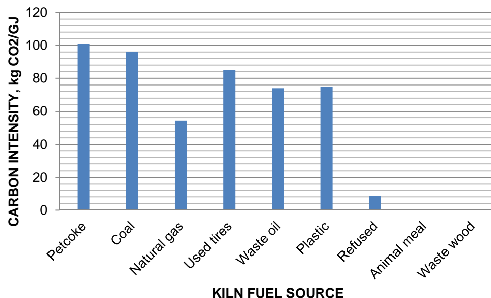
Figure 5 Intensity of emissions for various fuels
