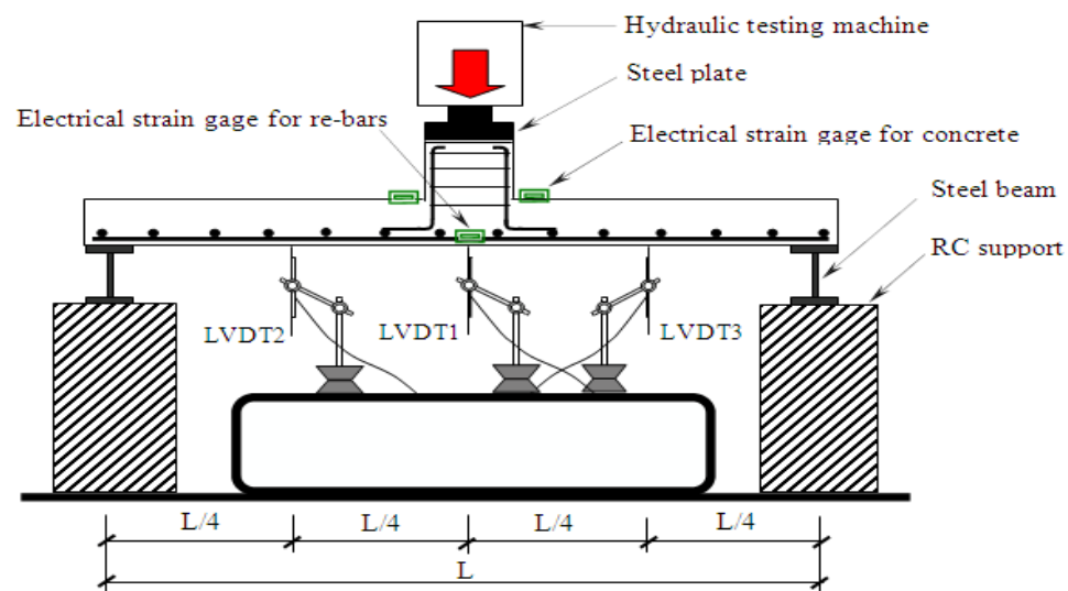
Figure 3 Test set-up
