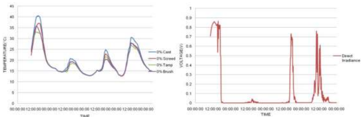
Figure 10 Time vs Temperature - 0% GGBS (left) and Corresponding Sunshine Data (right)
