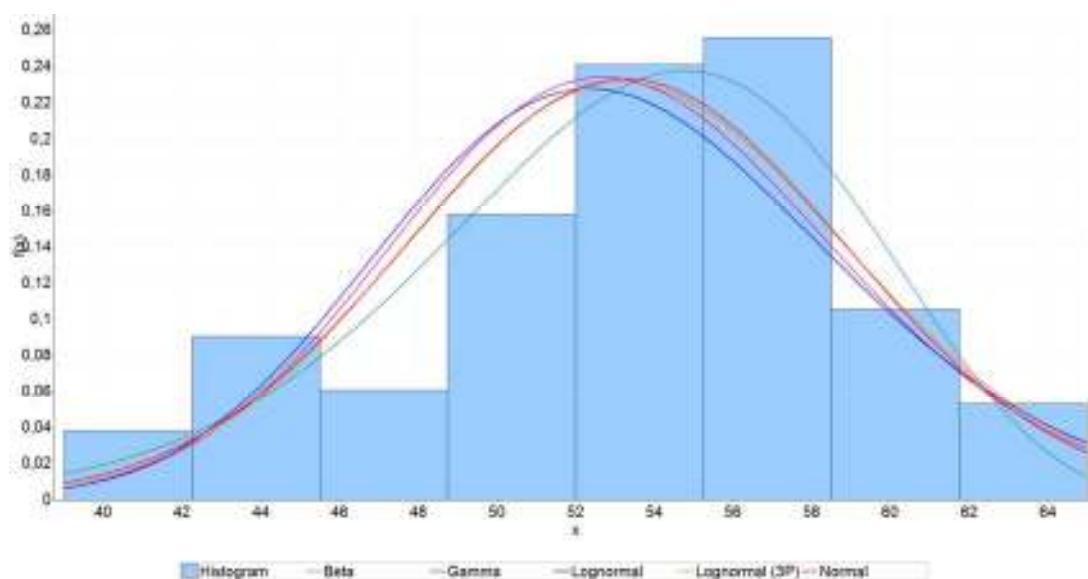
Figure 4 Histogram of compressive strength and the considered theoretical models
