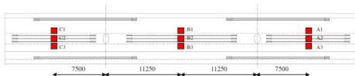
Figure 3 Locations of strain monitoring points (before strengthening)
