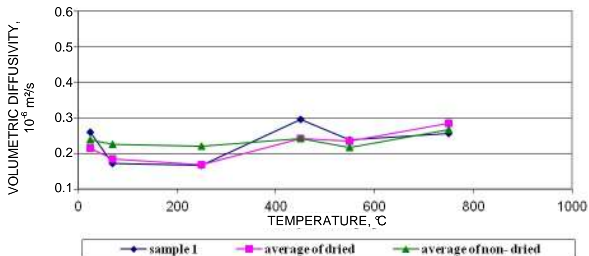
Figure 18 Thermal diffusivity dependence on temperature – RIGIBS
