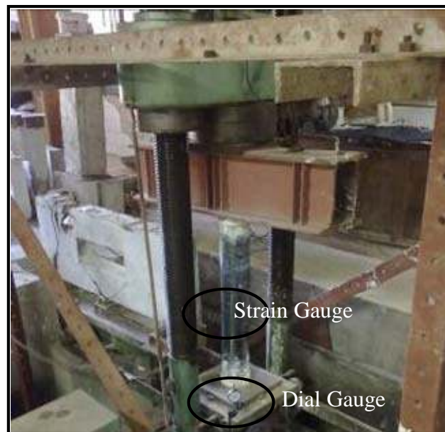
Figure 3 Test Setup and column instrumentation
