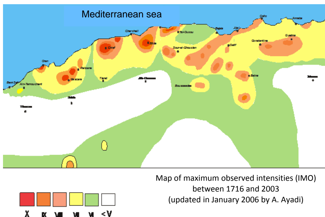
Figure 4 Maximum intensities in Algeria
