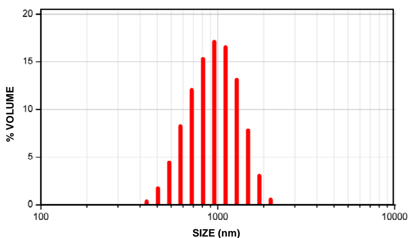
Figure 1 Particle size distribution of \text{TiO}_2 powder
