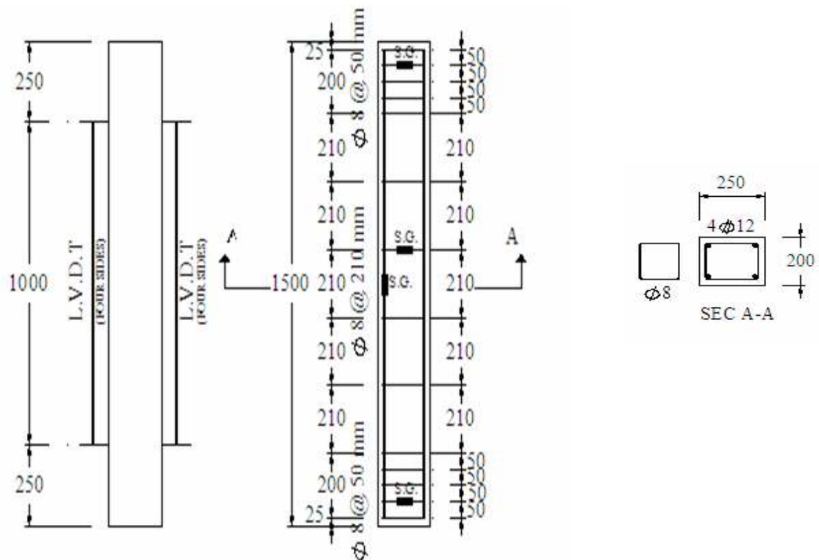
Figure 1 Concrete Dimensions of Tested Columns
