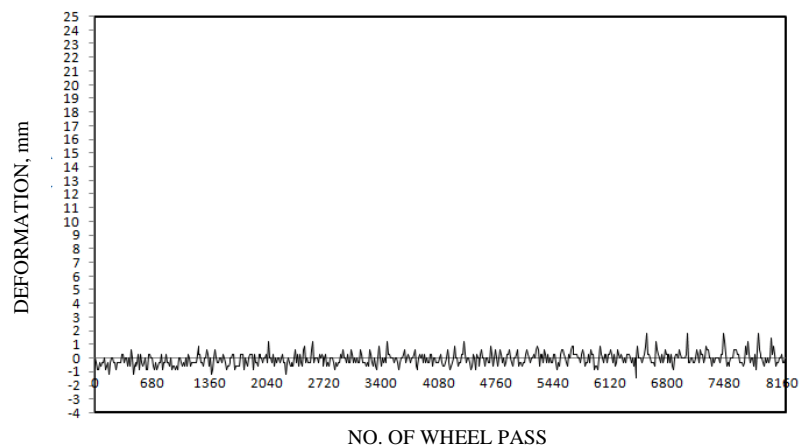
Figure 21 Typical test result for specimen with D503 mesh reinforcement
