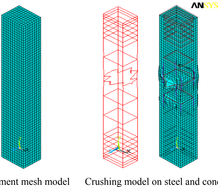
Figure 4 Finite element mesh for a typical column model and crushing model
