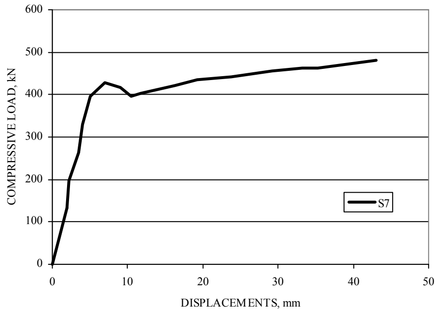
Figure 7 Compressive strength – Displacements
