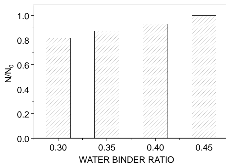
Figure 6 The quantity of dissolved \text{Ca}^{2+} of concrete with various water binder ratio
