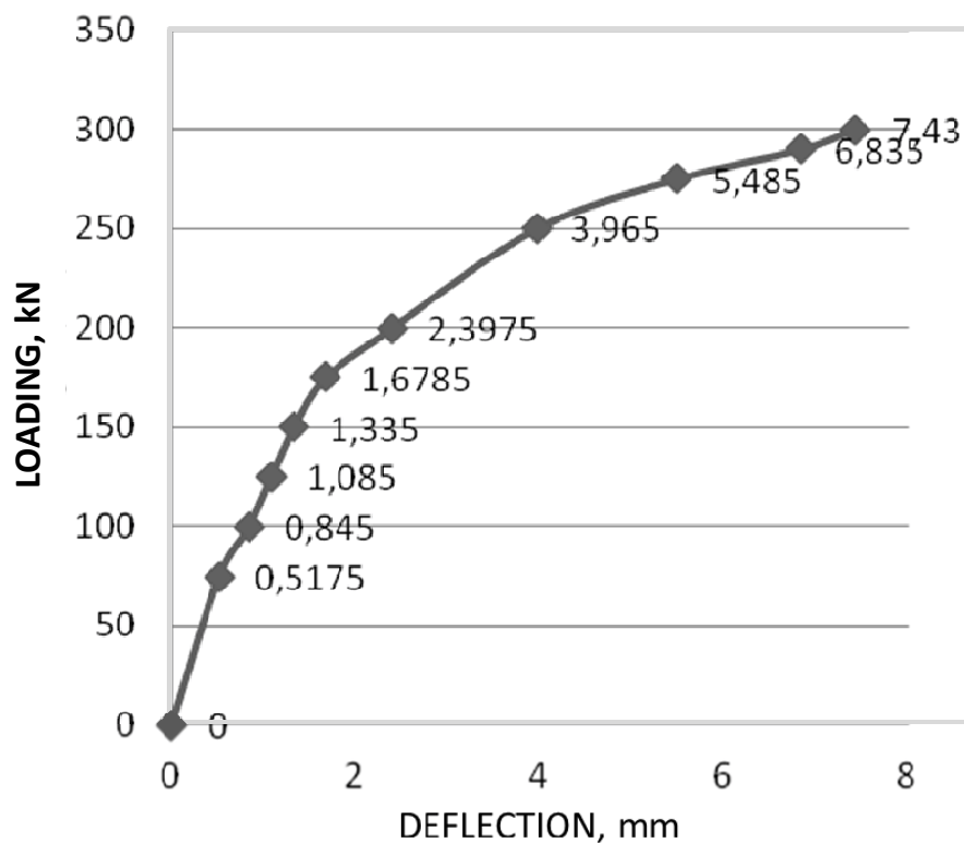
Figure 6 Loading-deflection diagram
