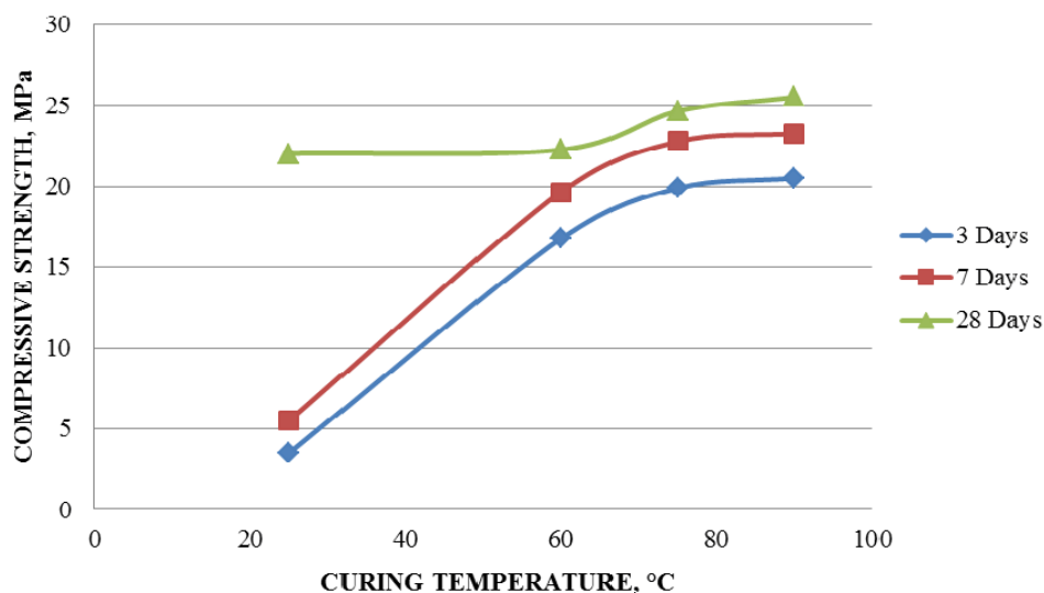
Figure 1 Effect of thermal activation temperature on strength of geopolymer concrete in hot air oven
