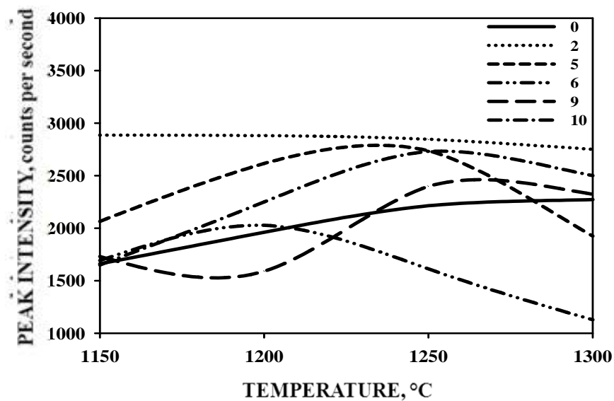
Figure2 XRD intensity of C_4A_3\bar{S} main peak for the burning products of the mixtures containing alumina powder vs. synthesis temperature (Mixture 0 is the reference mix based on natural materials)
