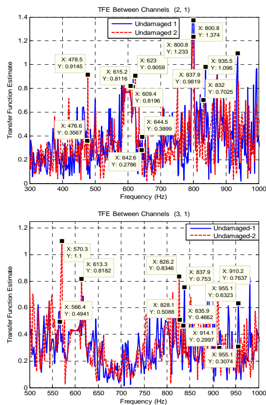
Figure 6 TFE for two tests on the undamaged structure
