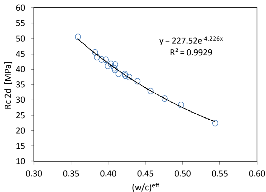
Figure 2 2-day compressive strength as a function of the effective w/c ratio.
