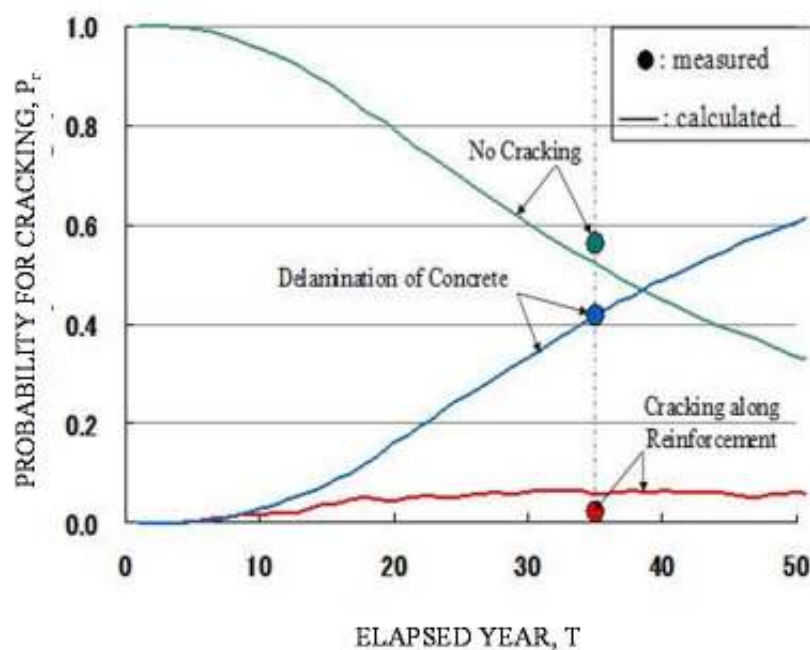
Figure 11 Cracking modes and elapsed year
