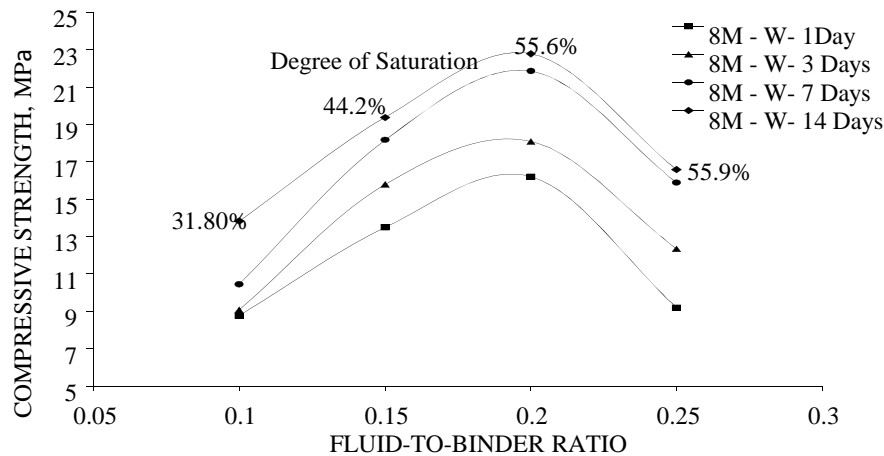
Figure 2 Compressive strength variation at constant density
