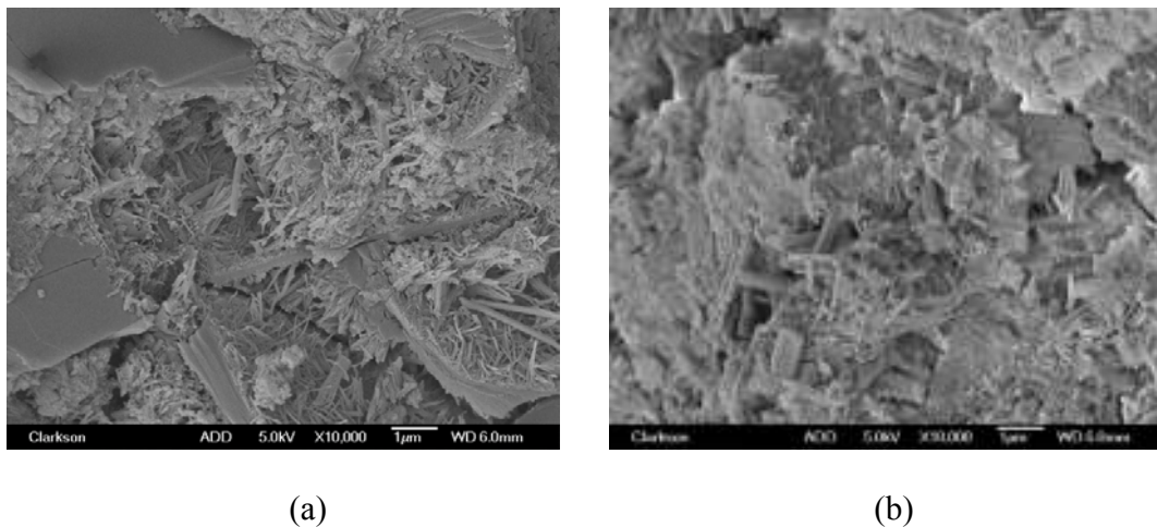
Figure 9 Micrographs of 20% CFBC fly ash modified pastes at (a) 14 days, and (b) 90 days of hydration
