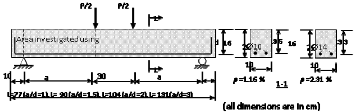
Figure 3 Geometry and reinforcement of beam
