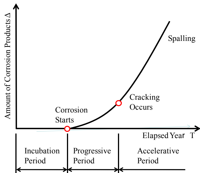
Figure 1 Relationship between corrosion rate and elapsed period
