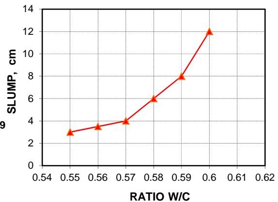
Figure 2 Effect of W/C on the workability on the compactness of sand concrete
