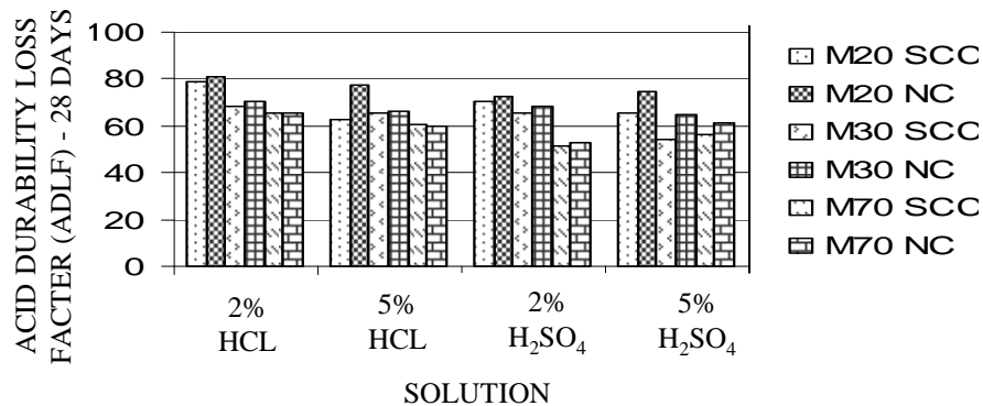
Figure 12 Acid Durability Loss Factors for SCC and NC at 28 days of immersion
