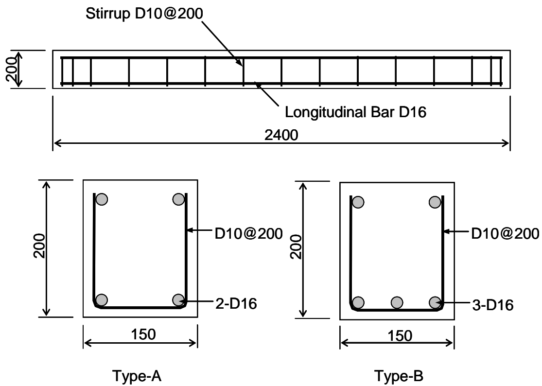
Figure 2 Specimen
