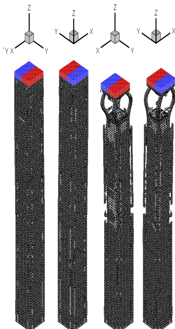
Figure 5 Fracture pattern in the ferroconcrete column of size 10\text{ cm} \times 10\text{ cm} \times 100\text{ cm} under loading that models endwise impact by 275 kg weight falling from 70 cm height
