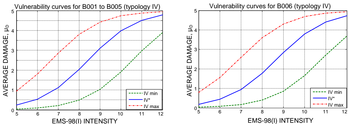
Figure 9 Vulnerability curves for building (B001...B006) calculated by the EU Risk method
