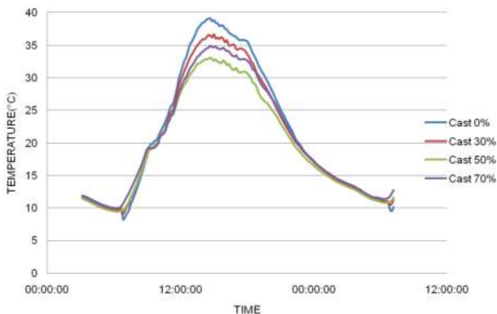
Figure 13 Time vs. Temperature - Cast Finish
