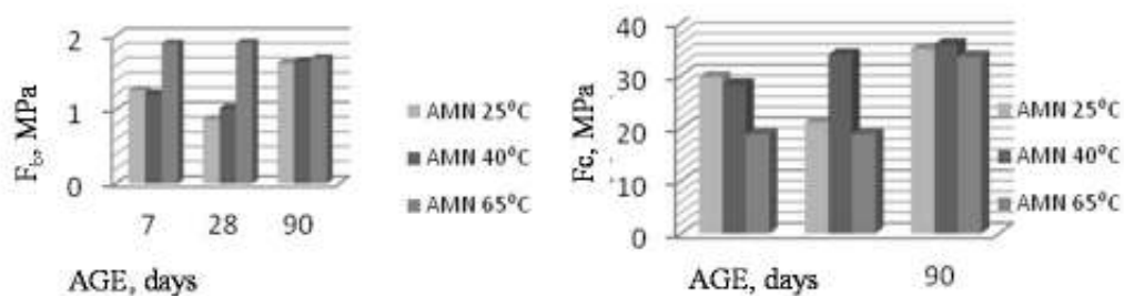
Figure 2 Flexural and Compressive strength of AMN 65% RH
