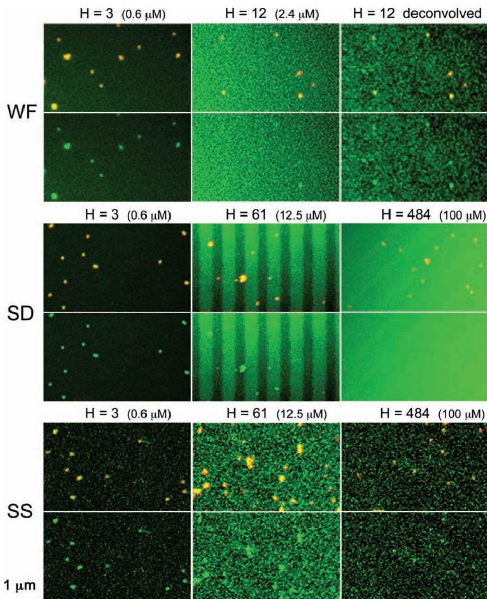
Fig. 3 Montage of images of beads with different amounts of out of focus fluorescence ( haziness index, H ) from wide-field (WF), spinning disk (SD) and spot scanning (SS) confocal microscopes. The concentration of AlexaFluor 488 in the background solution is given in parentheses for each image. For this figure, nonlinear contrast stretching has been employed to optimize single bead visibility in the green channel in the images with high background. The smallest objects visible in the red channel are single beads. Larger objects are clusters of multiple beads.
