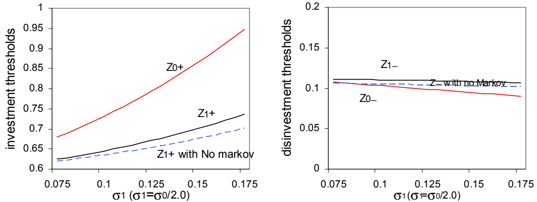
Figure 6: The Z Thresholds With and Without the Markov Switching Component
