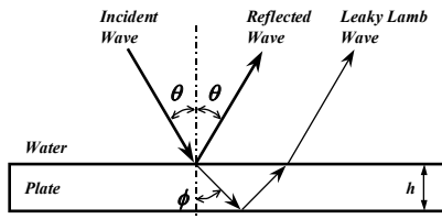
Fig. 1: Schematic of leaky Lamb wave.
