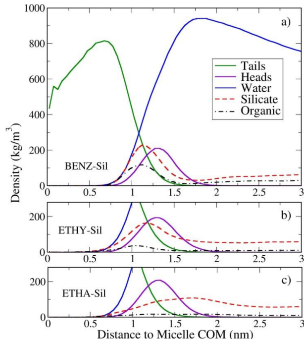
Fig. 2 Density profiles of micelles with \sim 20 surfactants formed in solutions with a) benzenesilica, b) ethylenesilica and c) ethanesilica.
