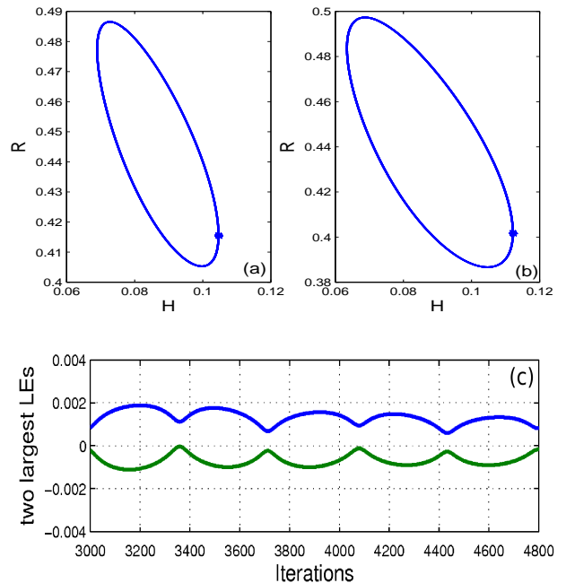
Figure 3: Phase space plot for the variables R and H , where the filled points is a Poincare map of the maximal values for the variable H . We consider the parameters according to Table 3, (a) \Delta = 0.01 and (b) \Delta = 0.025 . (c) Time evolution for the two largest Lyapunov considering \Delta = 0.025 .
