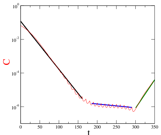
Figure 9: (Color online) Time evolution of the dimensionless quantity C according to the model (2) using (3), where we consider P = 10 and \Delta = 0.3 . The value of the first slope is -0.06 (black line), the second is -0.005 (blue line), and the third is 0.08 (green line).
