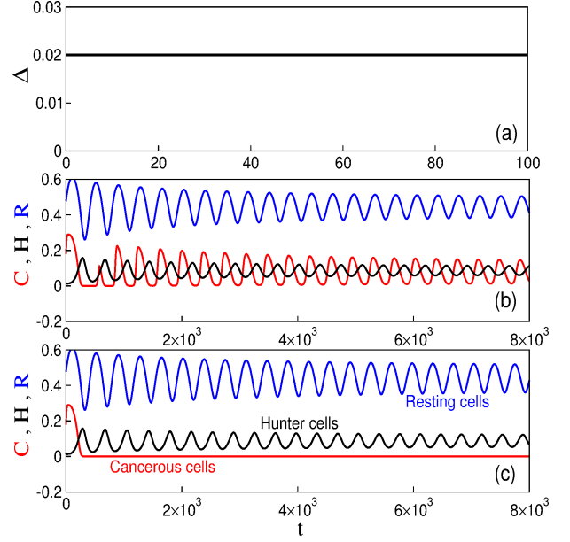
Figure 1: (Color online) Time evolution of the dimensionless quantities according to the model (2) using (3). (a) Continuous infusion rate of chemotherapy, (b) \Delta = 0.02 and (c) cancer suppression considering \Delta = 0.025 . The red line represents the cancerous cells, black line the hunter cells and blue line the resting cells.
