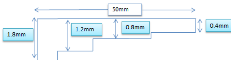
Figure 7 Thickness plate
