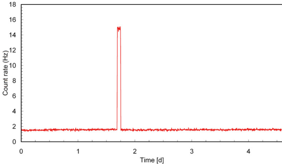
Figure 5. Bench test of the fiber sensor L30-2 over four and a half days. Three radioactive sources ( ^{60}\text{Co} , ^{137}\text{Cs} , ^{152}\text{Eu} ) with a total activity of 2.7 MBq were placed at \approx 8 cm from the fiber during two hours.
