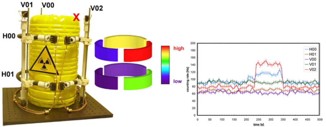
Figure 6. The prototype mini-drum with two horizontal and three vertical fibers. The “X” indicates the position where the gamma source was placed. The graph in the middle represents the 3D rough activity levels obtained by combining the horizontal and vertical information from the log data shown on the right.
