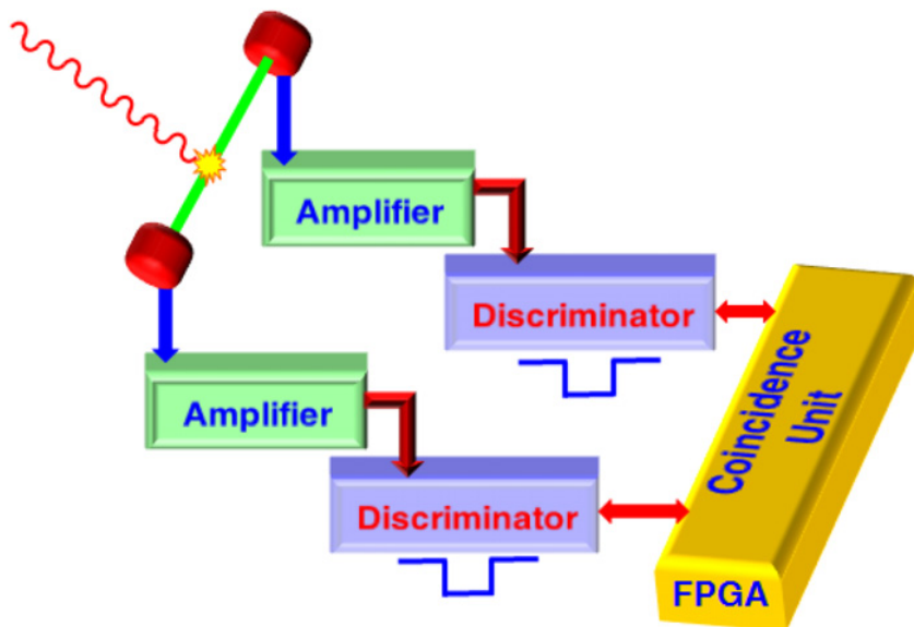
Figure 3. Scheme of the front-end electronics for one fiber. The output signal shape and type are represented near each component. It is worth to remark that a single FPGA can handle many fibers at once.
