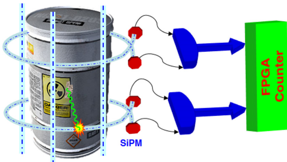
Figure 1. A possible layout of the fibres around the drum.
