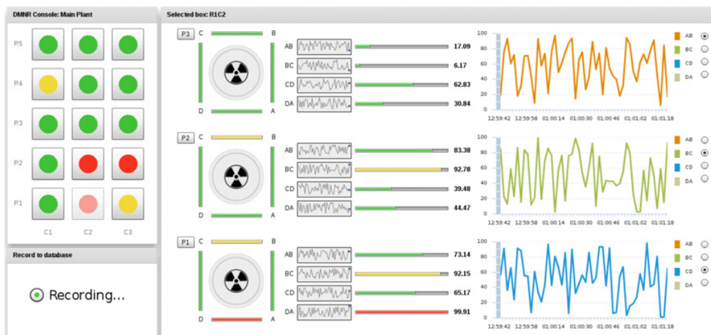
Figure 4. Graphical user interface.
