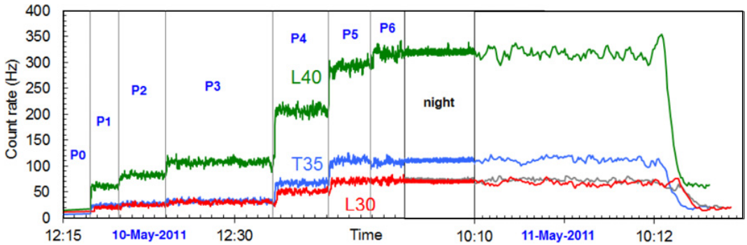
Figure 8. Counting rates as a function of time. First phase when the operator move the trolley along the seven positions, second phase the trolley is left in P6 position and at the and the quickly removal of the trolley.
