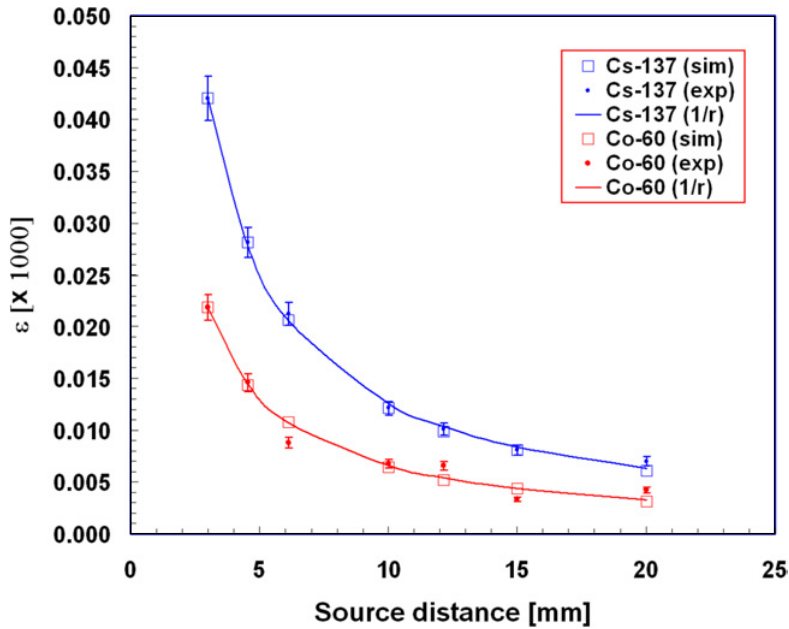
Figure 2. Detection efficiency of the fiber sensor to gamma radiation, as a function of the source distance, for two different sources: ^{60}\text{Co} and ^{137}\text{Cs} . Open squares: simulation; full circles: measured data; line: calculation assuming a 1/r dependence.
