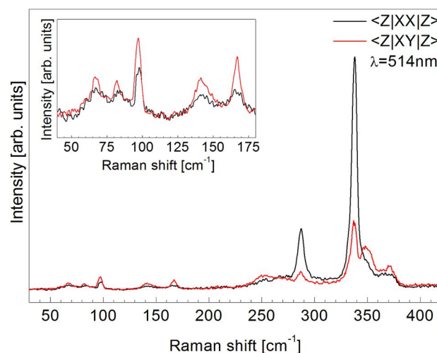
FIG. 3. Raman polarization measurements of \text{Cu}_2\text{ZnSnS}_4 done in parallel and perpendicular polarization configurations (excitation wavelength 514.5 nm).
