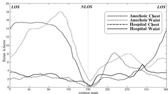
Fig. 4. Rician K-factor values versus rotation angle.
