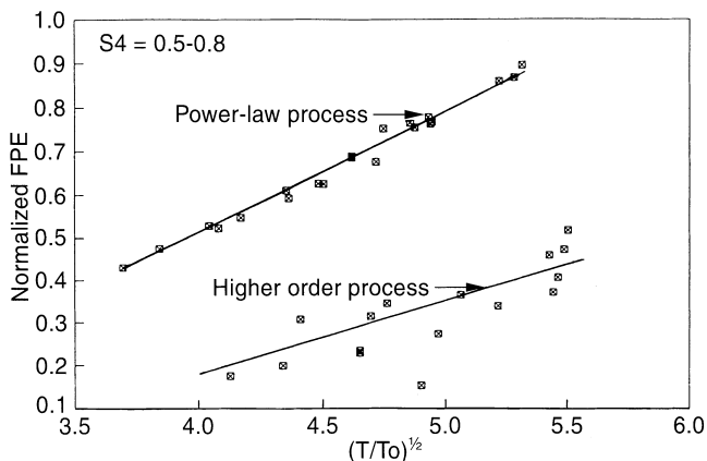
Fig. 10. This is a plot of the normalized final prediction error (obtained from AR algorithm based on Akaike criterion) versus the smoothing parameter (T/T_0)^{1/2} . The linear trend displayed by the power-law process indicates that the lower order processes are more amenable to smoothing than the higher order process due to the latter possessing in intrinsic coherence
