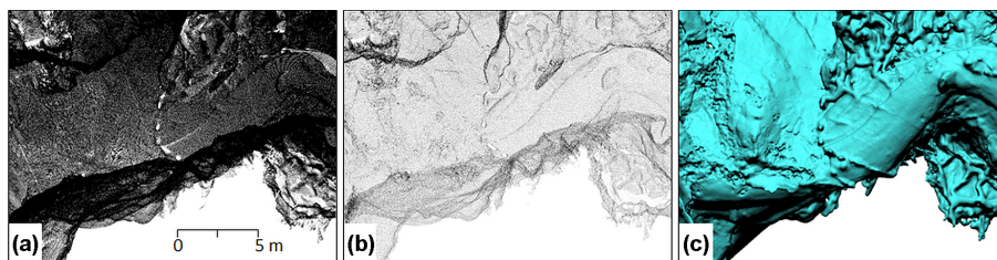
Figure 4. Point cloud from the Gothic Dome orthogonally projected on a horizontal plane representing 2 % of the full resolution as exported from the SCENE project (a), after subsampling the points at 5 cm minimal spacing (b), and as a continuous 3-D cave surface model (c) generated from (b) with the octree depth of 12.
