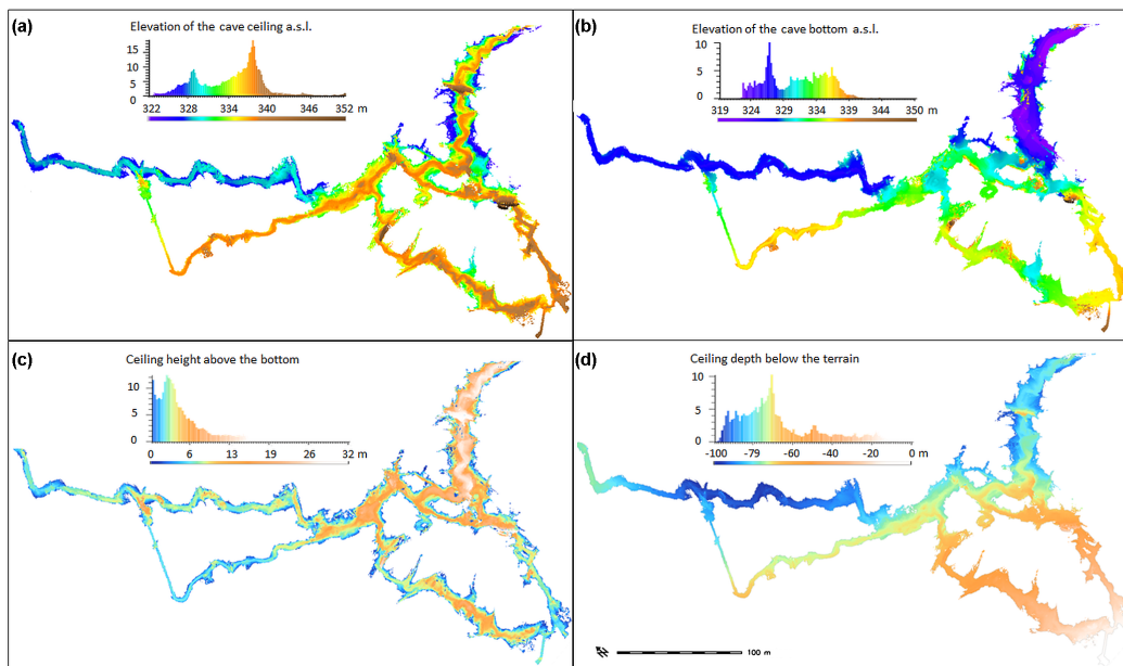
Figure 6. Raster based models with histograms representing the highest cave ceiling altitude (a), lowest altitude (b), vertical difference between the cave bottom and ceiling (c), and the ceiling depth below the terrain surface (d). The histogram y axis represents the number of raster cells in hundreds.
