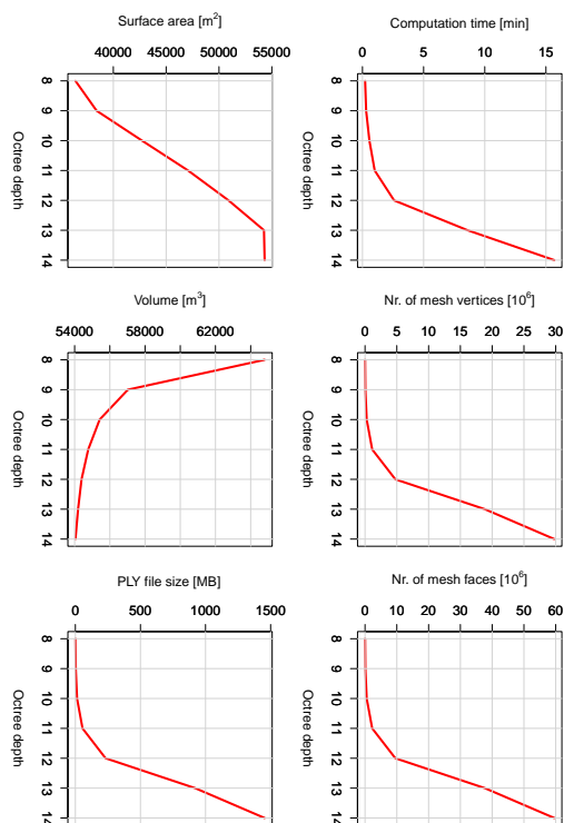
Figure 13. Relation between the octree depth parameter of the Poisson surface reconstruction in Meshlab and the associated computational time, number of vertices, number of facets, output mesh surface area, mesh volume, and file size. The input point cloud contained 12 718 million of TLS points representing the Domica cave which were processed on a desktop PC with the 64 bit Windows operation system, 16 GB RAM, and eight i7 CPUs of 3.6 MHz.
