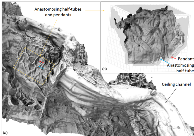
Figure 11. Ambient occlusion of the 3-D cave surface model in the Gothic Dome rendered with grey tones enhances perception of the cave surface morphology (a). Detail view of the smaller area of the 3-D mesh (b) shows the cave walls from inside. The size of the major and minor cells in the background grid is 1 and 0.5 m, respectively. The displayed mesh was generated from the original TLS data set subsampled at 1 cm point spacing demonstrating the high resolution of cave mapping.
