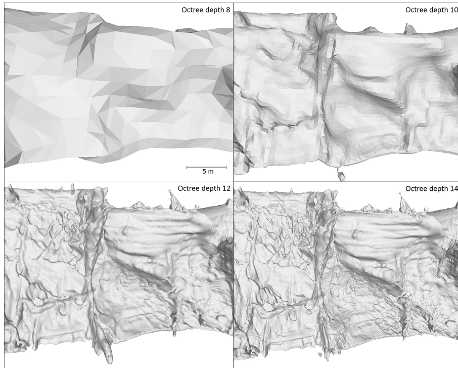
Figure 14. The level of detail for different 3-D meshes generated from the same input data with various octree depth parameter values of the Poisson surface reconstruction method. Example of the Gothic Dome using the input point cloud subsampled from the original at 5 cm minimal spacing.
