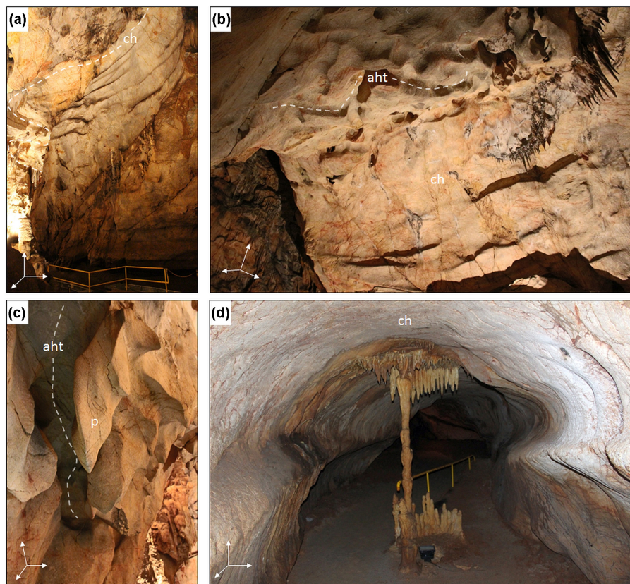
Figure 2. Examples of ceiling channels (ch), pendants (p), and anastomosing half tubes (aht) in the Domica cave as speleofoms associated with the phreatic regime. Presence of the speleofoms in the ceiling and walls of the Gothic Dome indicate paragenetic (antigravitational) development (a, b, c), while it is more difficult to infer from the “dry passage” ( Suchá chodba in Slovak) (d) from where much of the accumulated sediment was not evacuated and the passage was reshaped during multiple phases of vadose and phreatic conditions. The highest parts of the channels can be situated as high as 16 m (a, b) or 2 m above the floor on sediment accumulation (d).
