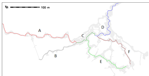
Figure 7. Segments of ceiling lines with assigned letters as referenced in the text and as reported in Table 5.
