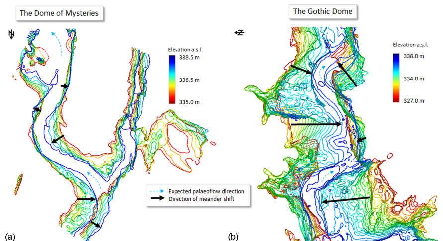
Figure 12. Elevation contours of the 3-D cave surface projected on a horizontal plane indicate upward migration of the ceiling meanders in the Dome of Mysteries (a) and in the Gothic Dome (b). Contour interval is 0.5 m.
