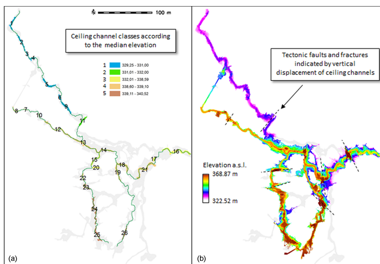
Figure 10. Ceiling channels resulting from the semi-automatic classification of the Domica ceiling, which were grouped according to their median elevation (a) reported in Table 6 and interpretation of their vertical displacement (b).
