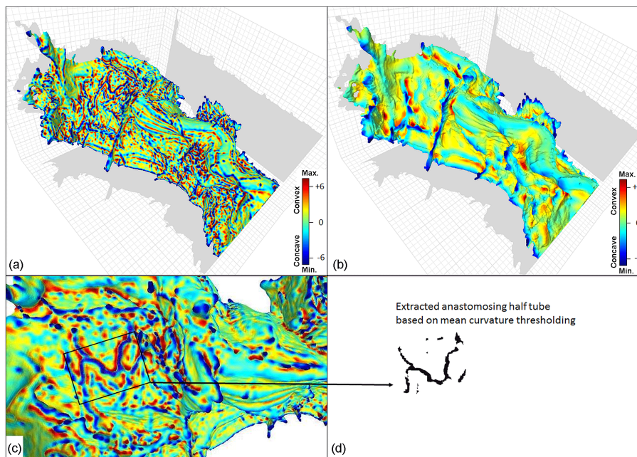
Figure 15. Mean curvature parameterization of the 3-D cave surface model in the Gothic Dome (Fig. 7a) at the scale of 5 (a), scale of 20 (b), selecting the surface of mean curvature between -8 to -3 \text{ m}^{-1} from (c), selected anastomosing half tube (d). The size of the major and minor cells in the background grid is 5 and 1 m, respectively. Orthogonal silhouette of the mesh is projected on the XY , XZ , YZ planes.
