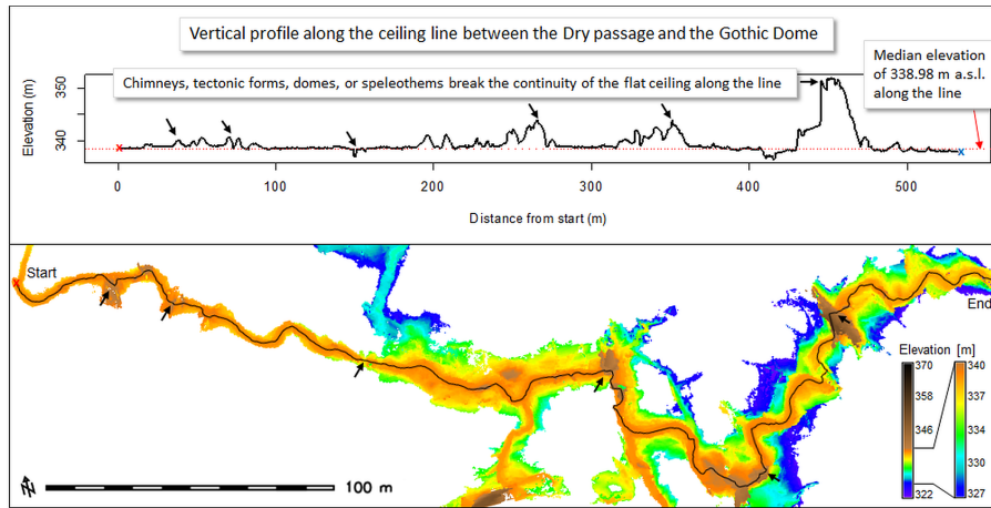
Figure 8. Longitudinal profile along the automatically delineated ceiling line of overlaid on top of the raster DEM_CH.
