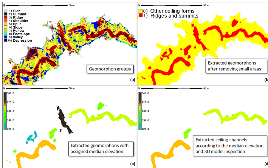
Figure 9. Classification of the ceiling surface (DEM_CH) of the Majko’s Dome and the Gothic Dome (Fig. 3) in GRASS GIS to extract the ceiling channels as landforms. Ceiling channels are classified with the r.geomorphons module as ridges and some parts as summits (a). The two categories are extracted as binary rasters with r.mapcalc and small clusters are removed with r.neighbors (b). The areas are clumped into individual spatial units for which elevation summary statistics were calculated. Median elevation (c) most appropriately separated the ceiling channels from other ridges and summits (d).
