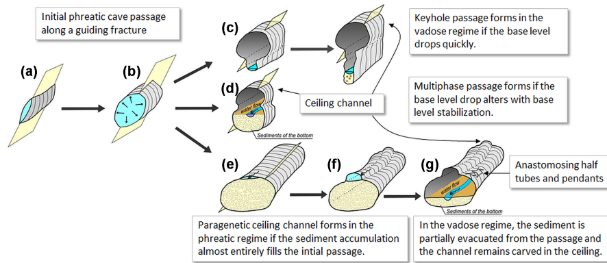
Figure 1. Schematic evolution of the passages in phreatic and vadose hydrological regime under conditions of high sediment flux and following abandonment (modified after Farrant and Smart, 2011). Further description of the stages is Sect. 2.1.
