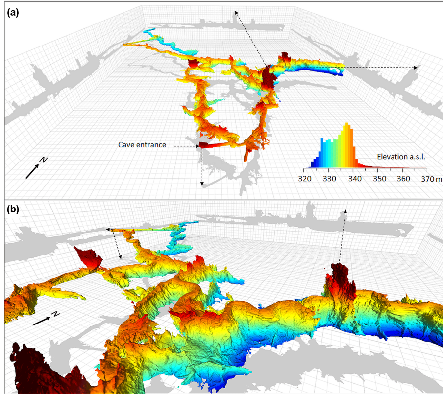
Figure 5. 3-D model of the Domica cave oriented towards the north (a) and its detailed view towards north-west (b) showing a meandering ceiling channel. The model is coloured by the value of altitude above mean sea level which distribution is shown by the histogram. The 3-D geometry is orthogonally projected on the XY, YZ, and XZ planes. The size of the major and minor cells in the background grid is 20 and 5 m along all three axes, respectively. Note the flat, horizontal ceiling levels projected on the vertical XZ and YZ planes.
