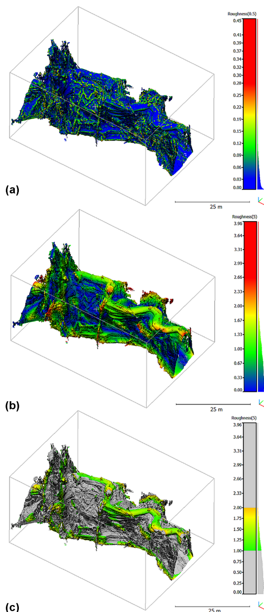
Figure 16. Roughness of the 3-D cave surface model in the Gothic Dome derived at 0.5 m scale (a), and 5 m scale (b), and selection of speleforms having values between 1 and 2 (c), respectively.
