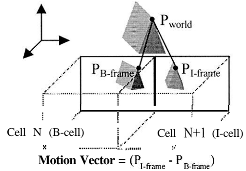
Figure 3: The motion vector associated with P_{B-frame} is calculated by back projecting the screen coordinates into world space ( P_{World} ) using depth information and then re-projecting P_{World} into screen coordinates for the reference frame ( P_{I-frame} ). The difference between these coordinates is a candidate motion vector for encoding the macroblock containing P_{B-frame} .
