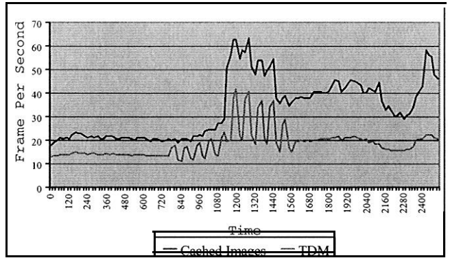
Figure 7: This graph highlights the frame rates through a sample path. We use spatial encoding to represent cached images as well as TDMs.
