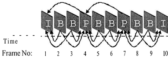
Fig. 2(a) Traditional MPEG Encoding
