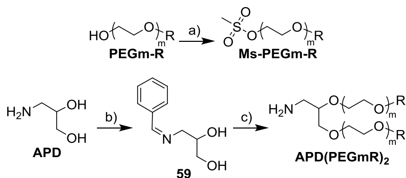
Scheme 4.10: Reagents and conditions: a) i. NEt 3 , DCM, 0 °C, 10 min, ii. MsCl, 0 °C – RT, 18 h; b) i. Na 2 SO 4 , DCM, MeOH, RT, 30 min, ii. PhCHO, RT, 18 h; c) i. NaH, THF, RT, 3 h, ii. Ms-PEG m -R , 67 °C, 17 h, iii. HCl (aq) , EtOH, 2.5 h. Yields are given in Table 4.04.
