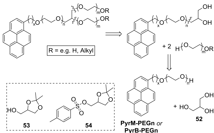
Figure 4.04: Retrosynthetic approach to an 'all-ether' podand surfactant derived from an 'anchor-linker' intermediate, glycerol ( 52 ) and OEGs. Suitable activation and protection of alcohol moieties would also be required, e.g. by using solketal, 53 , or its tosylate, 54 .
