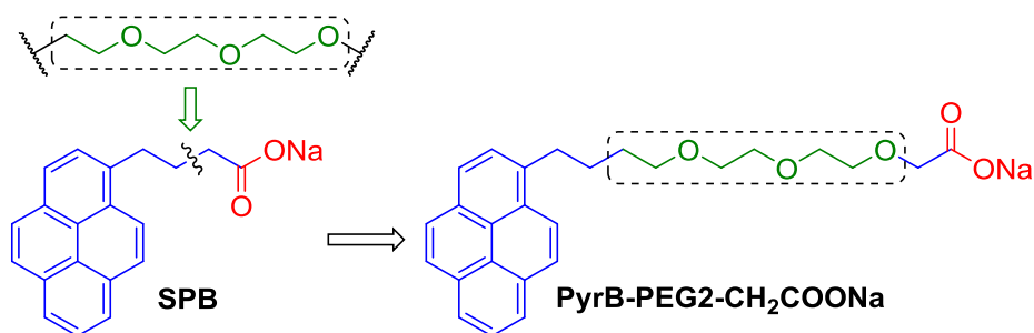
Figure 3.05: The structural difference between SPB and PyrB-PEG2-CH 2 COONa is equivalent to the addition of 3 PEG repeat units.
