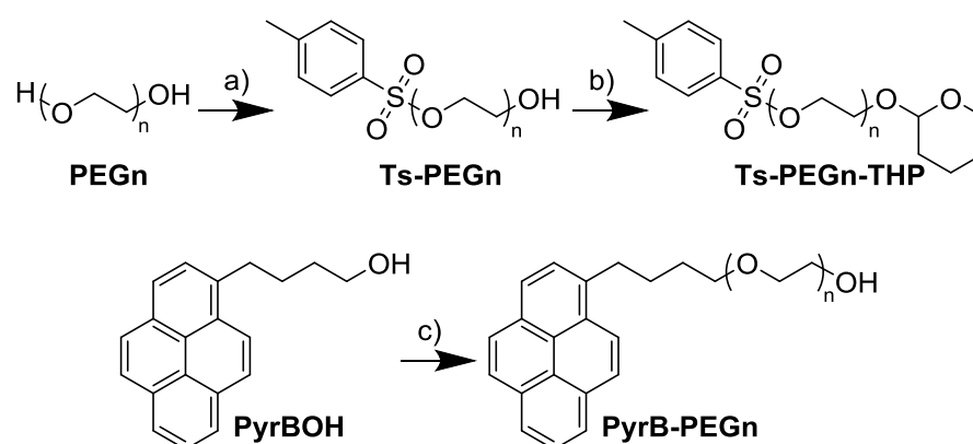
Scheme 2.25: Reagents and conditions: a) TsCl, Ag 2 O, KI, DCM, 0 °C, 15-60 min; b) pyridinium p -toluenesulphonate, dihydropyran, DCM, 40 °C, 20 h; c) i. NaH, THF, 67 °C, 1-2 h, ii. Ts-PEG n -THP , 67 °C, 18 h, iii. HCl/THF, RT, 18 h. Yields are given in Table 2.05.
