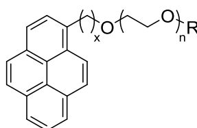
Figure 4.01: The general structures of targeted non-ionic surfactants. R represents a non-ionic, hydrophilic moiety.
