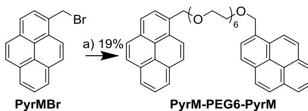
Scheme 2.14: Reagents and conditions: a) PEG6, NaH, THF, 40^\circ\text{C} , 2 h.
