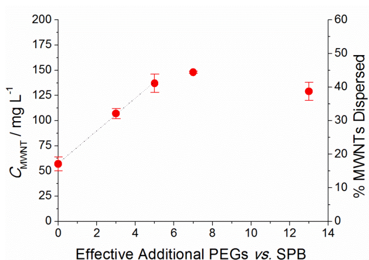
Figure 3.06: C_{\text{MWNT}} using 1 mM aqueous solutions of SPB and the series PyrB-PEG n -CH 2 COONa . Error bars are the standard deviation of 3 results except for SPB, where it is the standard deviation of 6 results.
