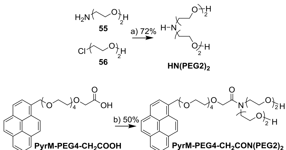
Scheme 4.06: Reagents and conditions: a) Na 2 CO 3 , toluene, 110 °C, 96 h; b) i. DIPEA, TBTU, DCM, RT, 15 min, ii. HN(PEG2) 2 , RT, 72 h.
