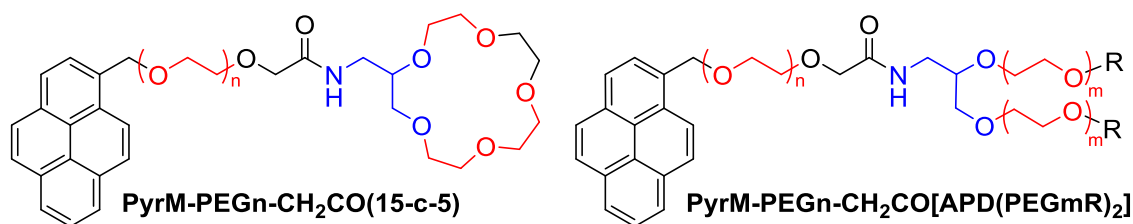
Figure 5.06: The total number of PEG repeat units in a surfactant, p , was defined by counting the units highlighted in red for crown ether (left) and podand (right) surfactants, respectively. For consistency no part of the APD moiety (highlighted in blue) was included in this count.
