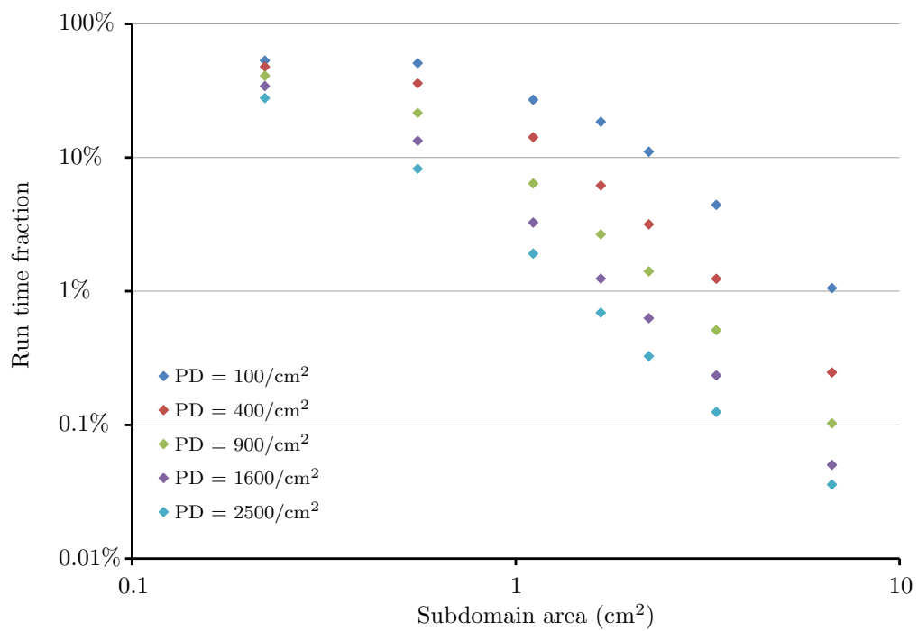
Figure 6.2: Change in the fraction of run time required by the solution of Algorithm 6.1 with subdomain area for a single, no flow reaction step in a 9cm by 9cm domain at a range of initial particle densities.
