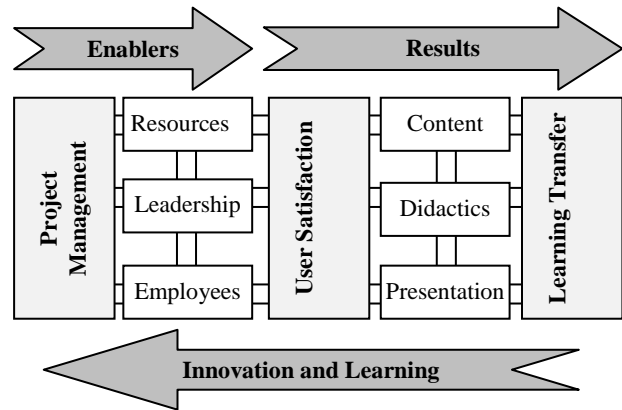
Fig 5: eValue-model
