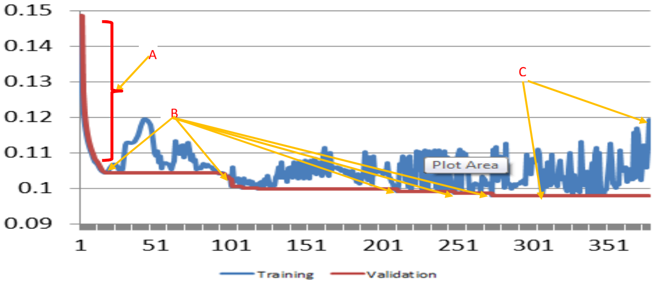
Figure 2 Evolution of the Training Error
