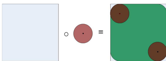
Figure 3. Opening of a square by a disk
