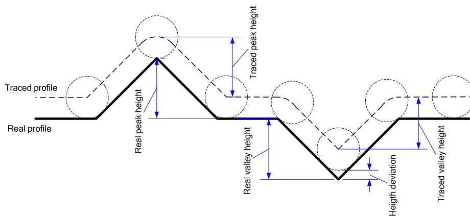
Figure 6. Tip mechanical filtering effects
