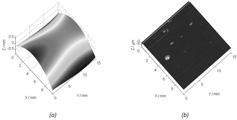
Figure 1. The measured F -theta surface (a) and the residual surface (b) generated by the morphological closing operation with ball radius 3 mm, which clearly presents machining marks.
