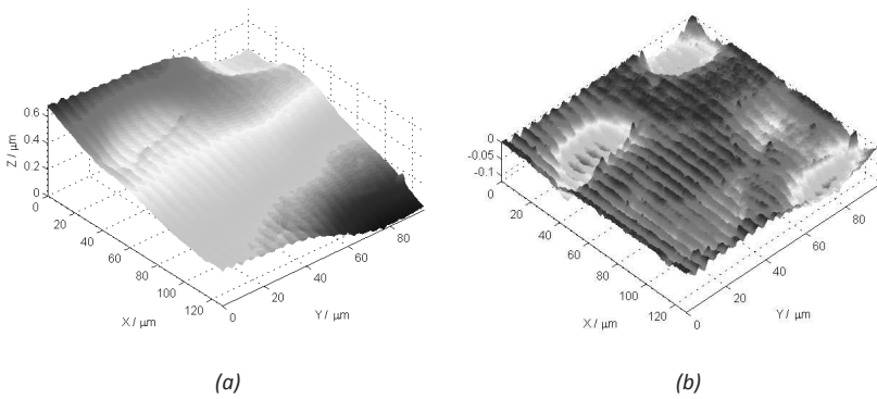
Figure 2. The measured tooth implant surface (a) and the residual surface (b) generated by the morphological closing operation with ball radius 10 mm, which evidently presents sand-blasting marks.
