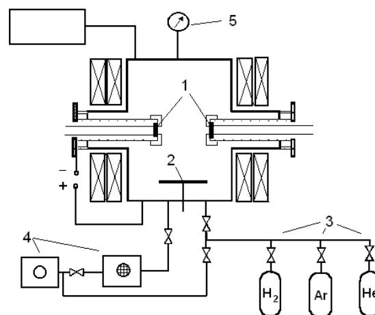
Fig. 1 – Schematic representation of the experimental facility for making the samples by plasma evaporation-sputterings: 1 – cathodes of metals to be sputtered – Mg and Ti; 2 – sample holder; 3 – gas bottles; 4 – pumps; 5 – pressure meters
