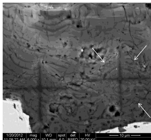
Fig. 6 – SEM image of microstructure of \text{Al}_2\text{O}_3 coating with measuring microhardness ( \text{HV}_{0.3} )
