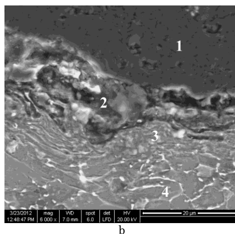
Fig. 4 – Structure of Al 2 O 3 coating (SEM)
