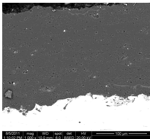
Fig. 2 – Microstructure of transverse sections of the sample with coating of Al 2 O 3
