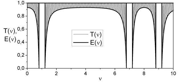
Fig. 1 - Spectral dependencies T(\nu) and E(\nu) of the filter (8) at n_A = 2.3, n_X = 2.89, n_B = 1.67, n_Y = 1.338, n_S = 1.5, N = 10
