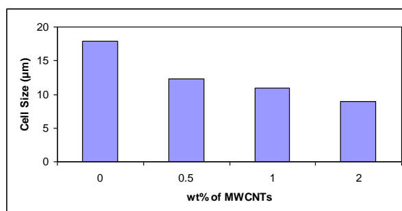
Fig. 4 – Effect of weight percent of CNT on average cell size of microcellular foams
