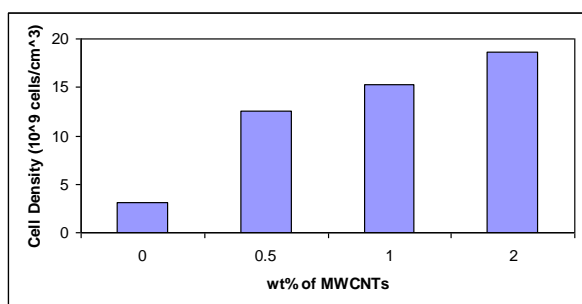
Fig. 3 – Effect of weight percent of CNT on cell density of microcellular foams
