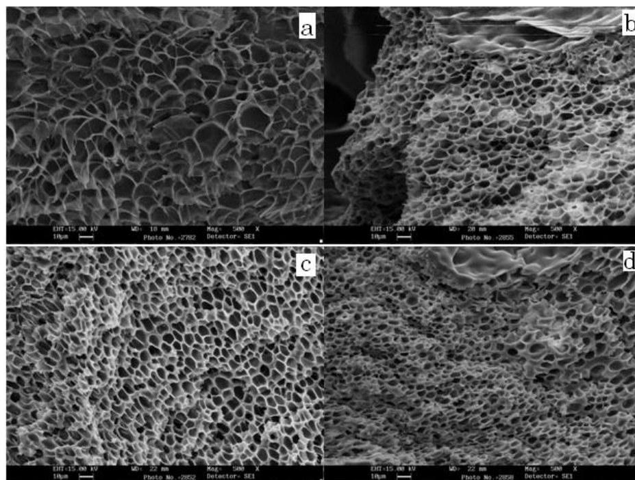
Fig. 2 – Scanning Electron Microscopy of microcellular foams prepared from nanocomposites with amount of 0 (a), 0.5 (b), 1 (c) and 2 (d) weight percent of CNT, The scale bar is 10 \mu\text{m} .
