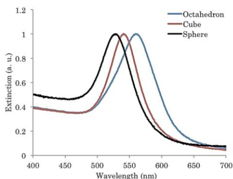
Fig. 2 – Extinction spectra of aqueous solutions of gold nanoparticles employed in this study
