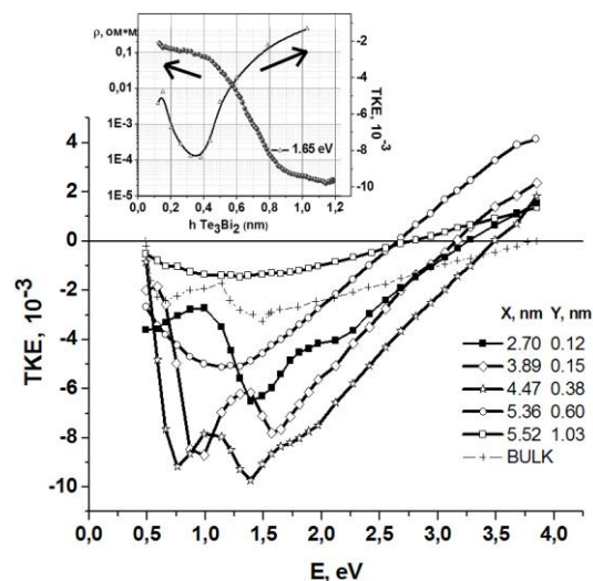
Fig. 1 – Spectral dependencies of TKE for [(\text{Co}_{40}\text{Fe}_{40}\text{B}_{20})_{33.9}(\text{SiO}_2)_{66.1}]/(\text{X nm})/[\text{Te}_3\text{Bi}_2](\text{Y nm}) multilayer samples. On the inset there are TKE and specific resistance \rho dependencies from thickness h of semiconducting spacer \text{Te}_3\text{Bi}_2
