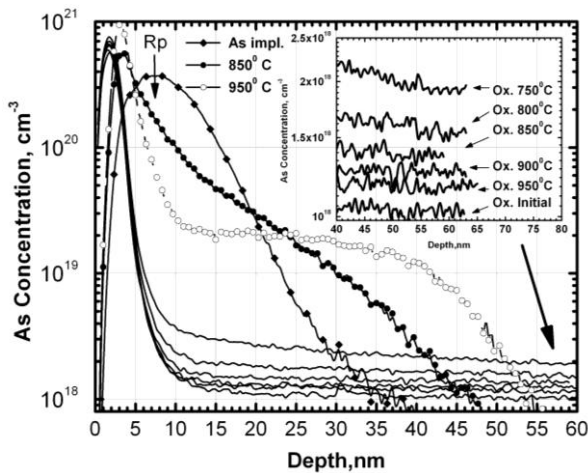
Fig. 1 – SIMS depth profiles comparing the temperature dependence of diffusion and segregation of background oxygen and As for 5 keV implantation through a 2.5 nm oxide.
