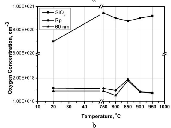
Fig. 2 – Oxygen concentrations at the screening SiO 2 , arsenic projected range (Rp) and arsenic tail (60 nm) regions of Si for As implantation energy 5 keV (a) and 10 keV (b) in dependence on temperature.
