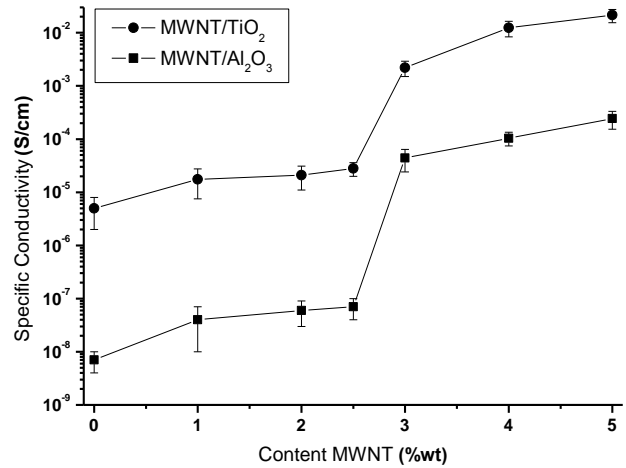
Fig. 2 – Dependence of the conductivity of the composites MCNT/Al 2 O 3 and MCNT/TiO 2 on the mass content of carbon nanotubes
