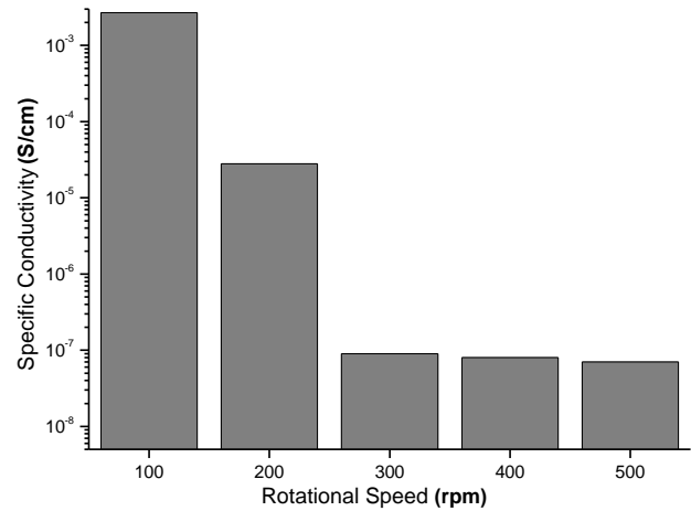
Fig. 3 – Dependence of the conductivity of the composites TiO 2 /MCNT (3%wt) on the number of revolutions
