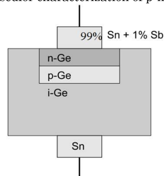
Fig. 1 – Schematic illustration of irradiated i-Ge sample with p-n junction and soldered contacts
