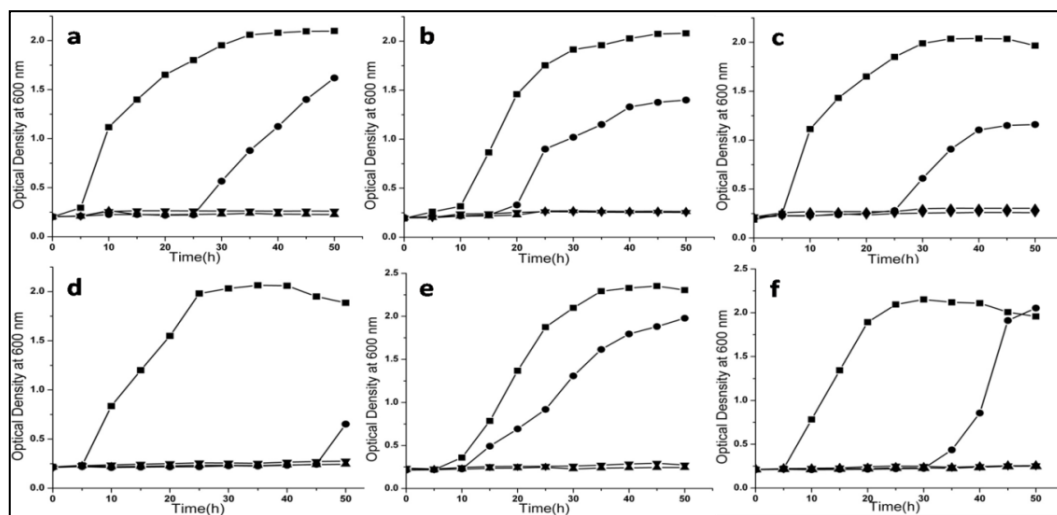
Fig.5. Antimicrobial activity of silver nanoparticles on a) E.coli , b) Enterococcus faecalis , c) Staphylococcus aureus , d) Klebsiella pneumoniae , e) Pseudomonas aruginosa and f) Proteus vulgaris with different concentration as \blacksquare control, \bullet 30 \mu\text{g/ml} , \blacktriangle 50 \mu\text{g/ml} , \blacktriangledown 100 \mu\text{g/ml}
