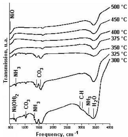
Fig. 2 – IR-spectra of nickel acetate hexaamine decomposition products obtained at different temperatures
