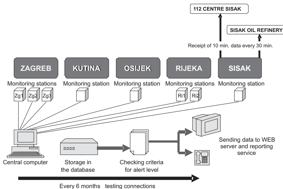
Fig. 1. Scheme of automatic data and information transfer from the point of measurement to the customer as designed in the State network for air quality monitoring. Source: EKONERG.
