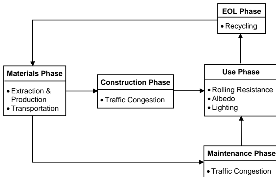
Figure 2: Proposed system boundary for road project LCA study.
