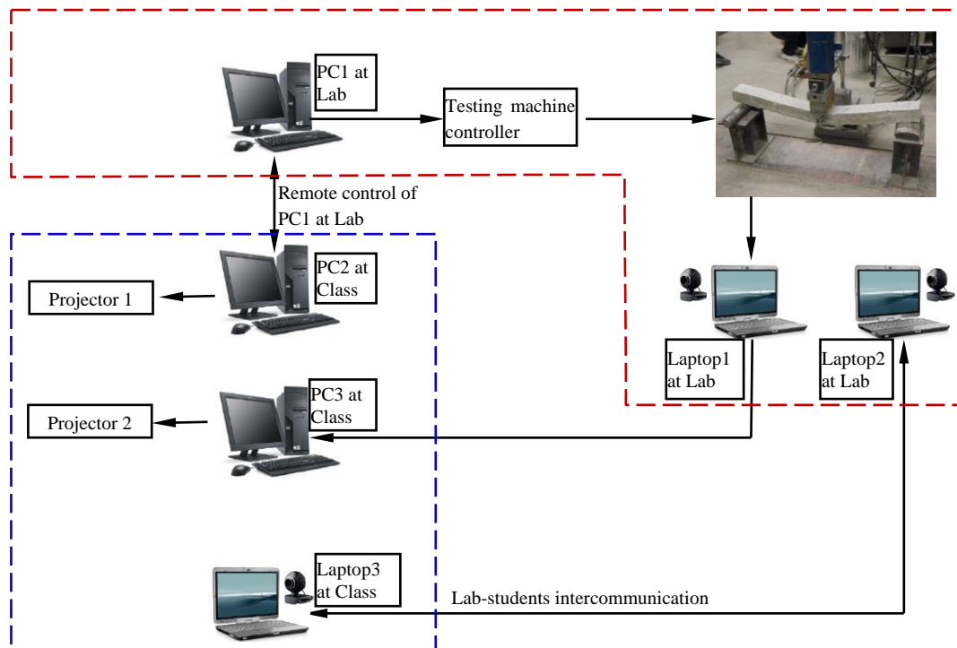
Figure 1: Schematic setup of the remote laboratory experimentation.
